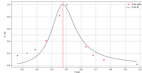
Figure 10: P/P_0(f) a 0.9A
