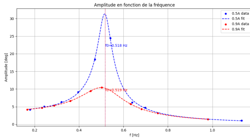
Figure 8: Amplitude(f)
