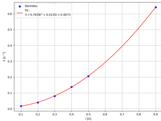
Figure 5: \lambda(I)
