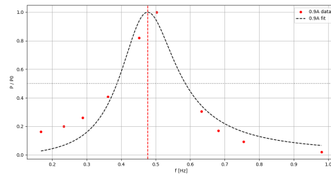
Figure 9: P/P_0(f) a 0.9A
