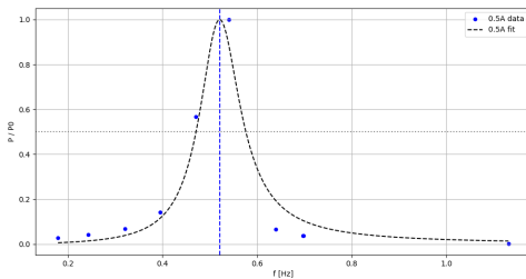
Figure 8: P/P_0(f) 0.5A
