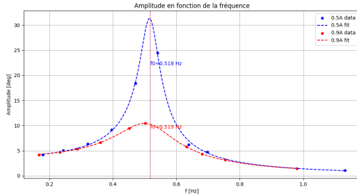
Figure 7: Amplitude(f)
