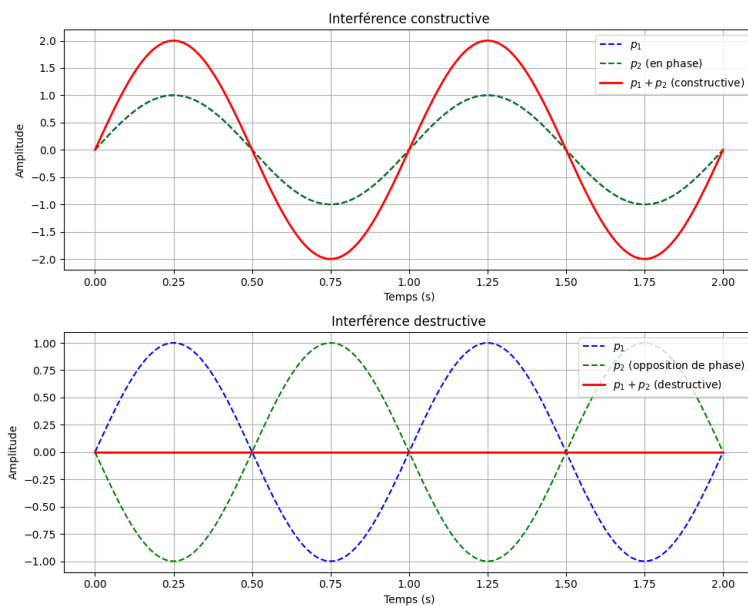
FIGURE 5 – Illustration d'ondes constructives et destructives.
