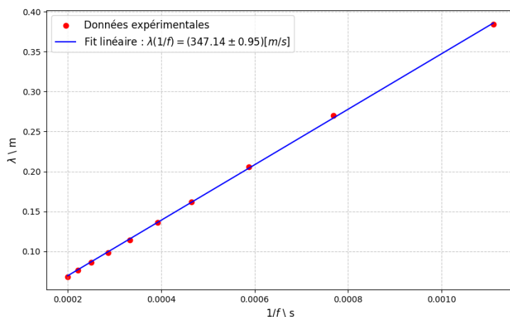
FIGURE 3 – \lambda(T)
