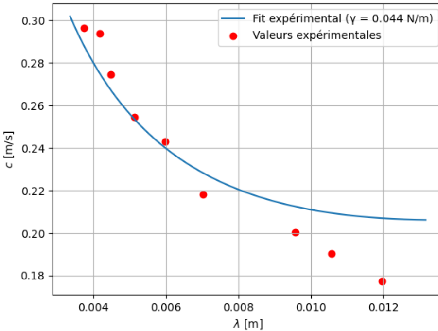
FIGURE 6 – v_\phi(\lambda)
