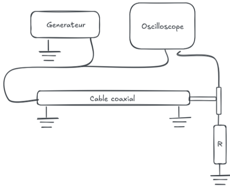
Figure 7: Montage experience cable coaxial
