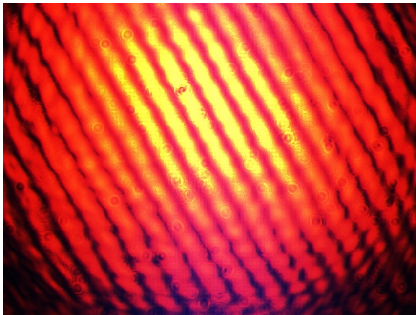
Figure 17: Interferances
