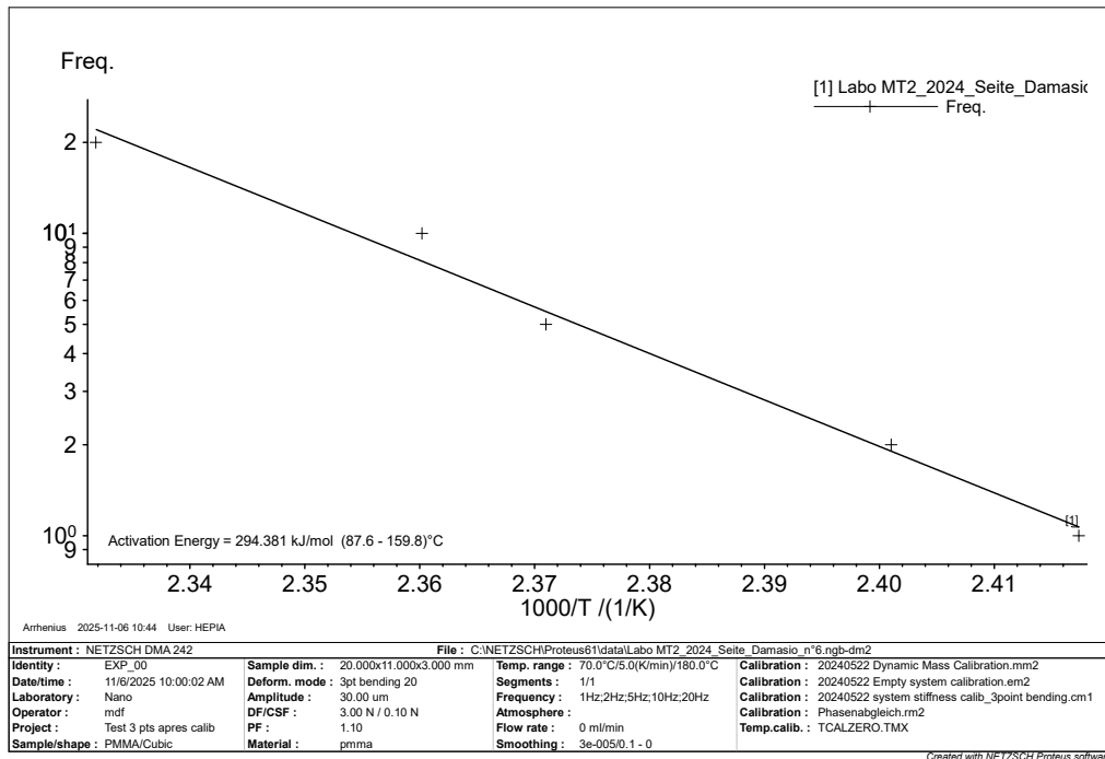
Figure 10: Arrhenius graph
