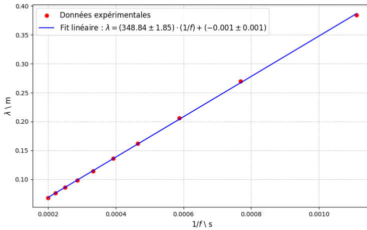
FIGURE 4 – \lambda(T)
