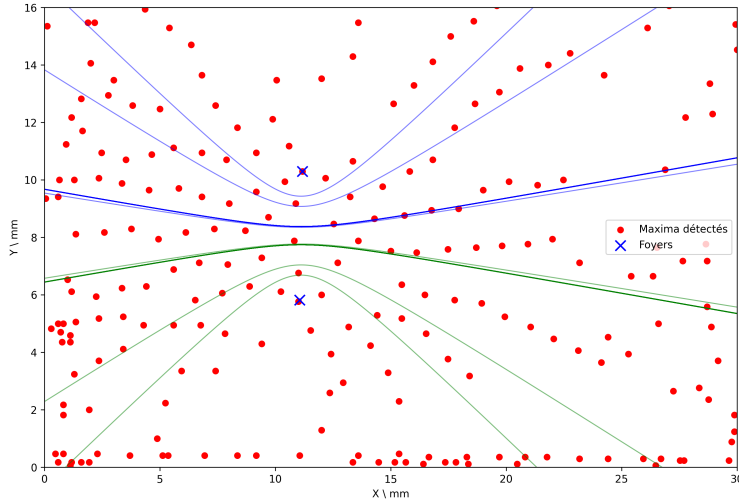
FIGURE 8 – Z_L = 2000\Omega
