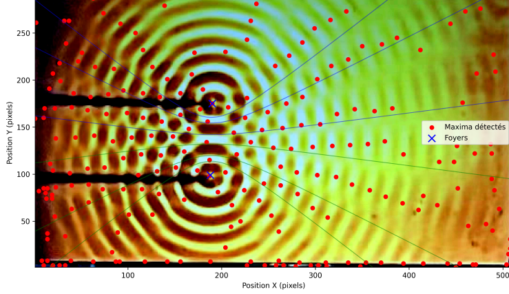
FIGURE 7 – Z_L = 2000\Omega
