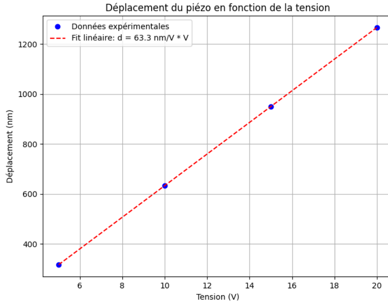
Figure 10: Coefficient piezzo-electrique
