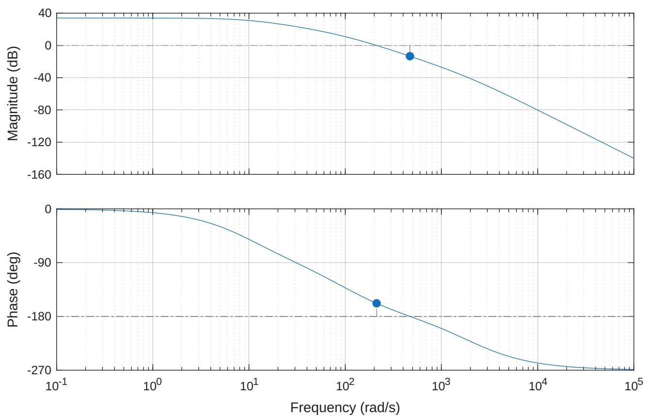
Bode de G_0(s) = G_s(s) avec K_p = 1 G_m = 13.3 dB (at 470 rad/s), P_m = 21.9 deg (at 212 rad/s)
