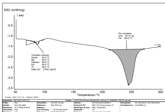
Figure 6: \delta H(T[^\circ\text{C}]) chauffe rapide
