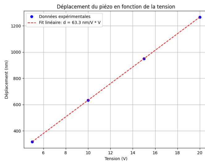
Figure 11: Coefficient piezzo-electrique
