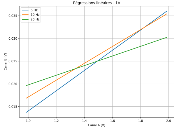
Figure 4: Z_L = 2500\Omega
