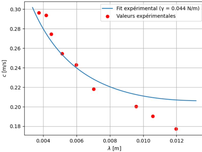
FIGURE 6 – v_\phi(\lambda)
