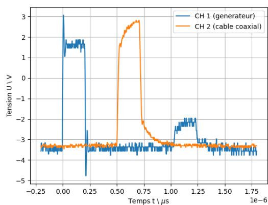
Figure 12: Z_L = 100 \Omega
