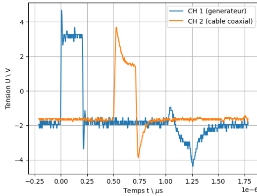
Figure 10: Z_L = 25 \Omega
