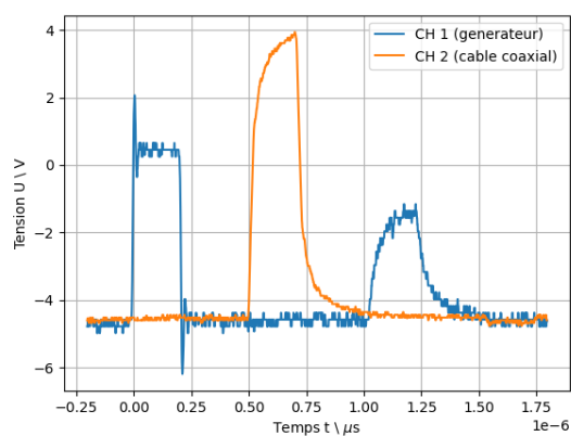
Figure 13: Z_L = 500 \Omega
