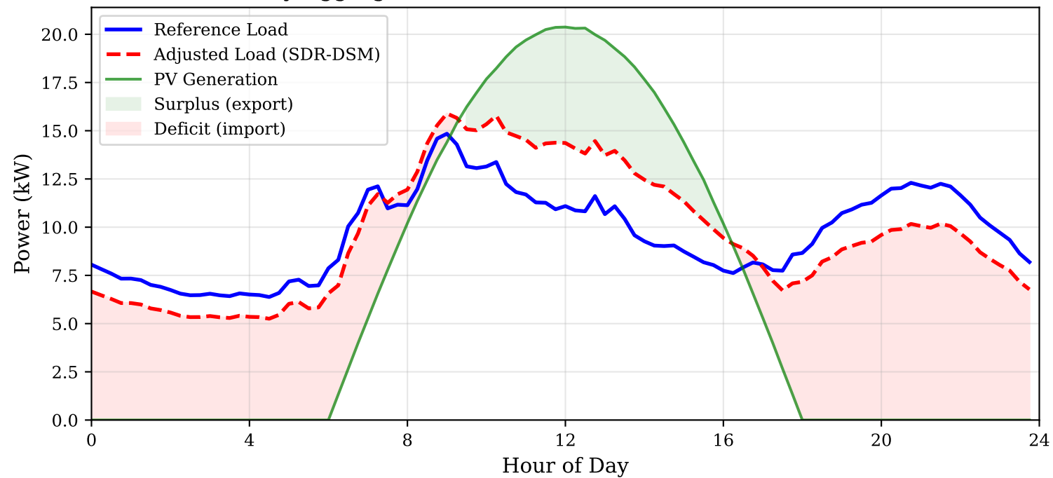
Community Aggregate Profile (56 Real Indian Meters, 60% Prosumer)
