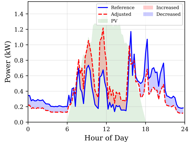
Prosumer A (High PV)
