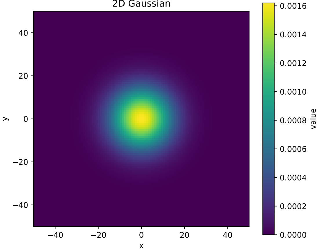
2D Gaussian
