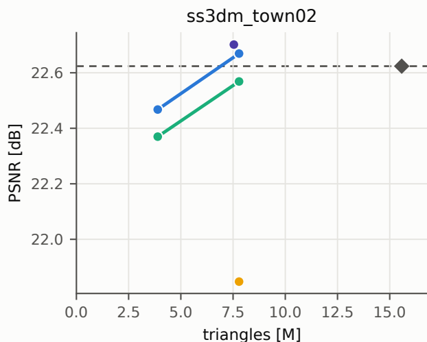
F2 — Pareto: PSNR [dB] vs triangle count (SGEO); budgets B12.5/B25/B50; dual anchors
