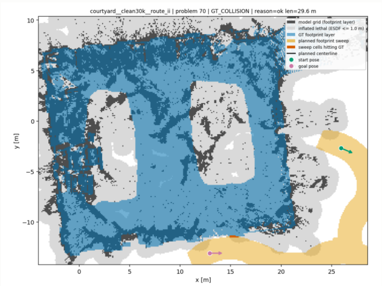
(c) maneuver example — courtyard route-ii plan sweeps a GT wall its grid marks free (R3.c panel; grid bit-identical clean↔B50)
