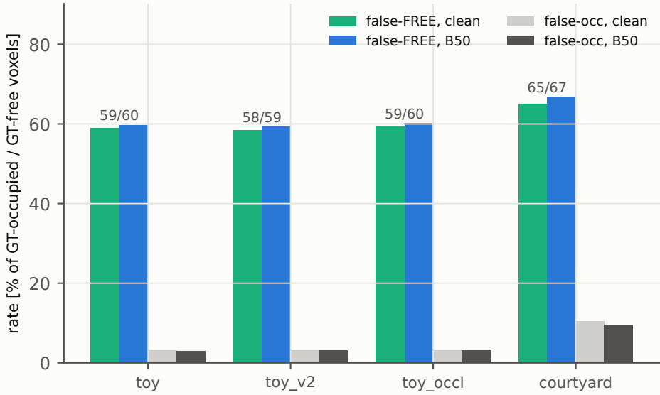
(a) d1 occupancy confusion @0.10 m — B50 PRESERVES the clean model's (bad) confusion; false-free is safety-critical
