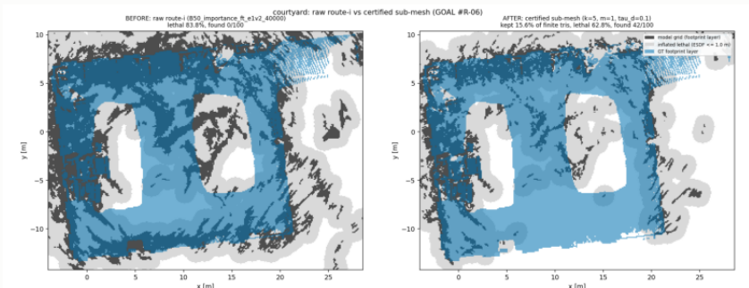
(d) R3.b certification sheds load-bearing surface — courtyard footprint before/after (kept set EXACTLY identical clean↔B50)
