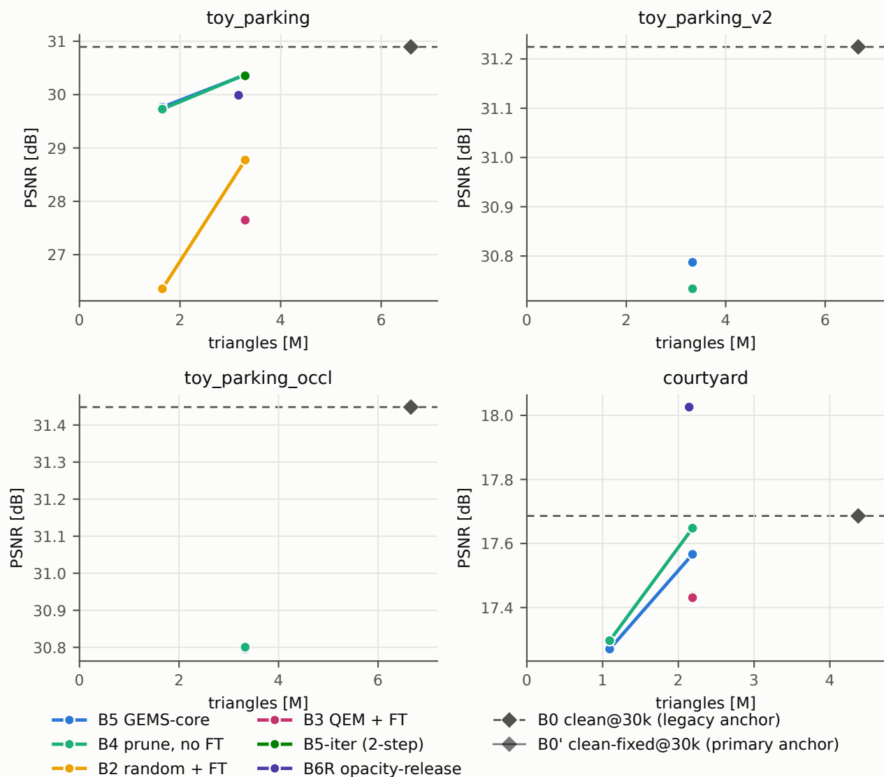
F2 — Pareto: PSNR [dB] vs triangle count (SDEV); budgets B12.5/B25/B50; dual anchors
