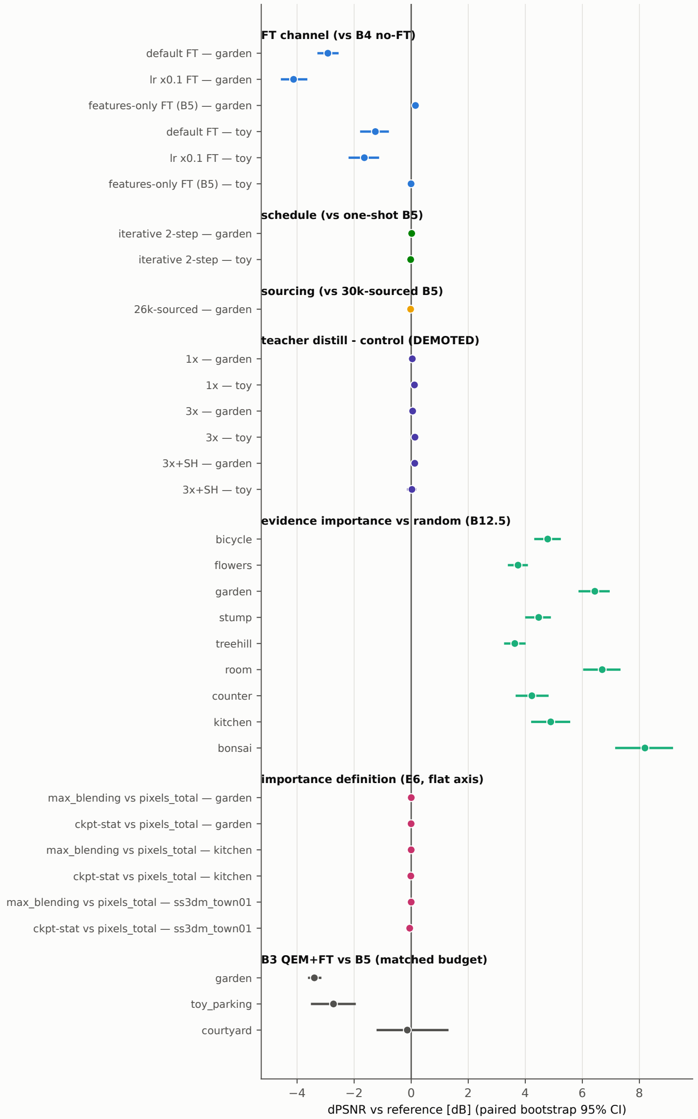
F7 — Ablation deltas (E6 mapping of Stage-One variants)
