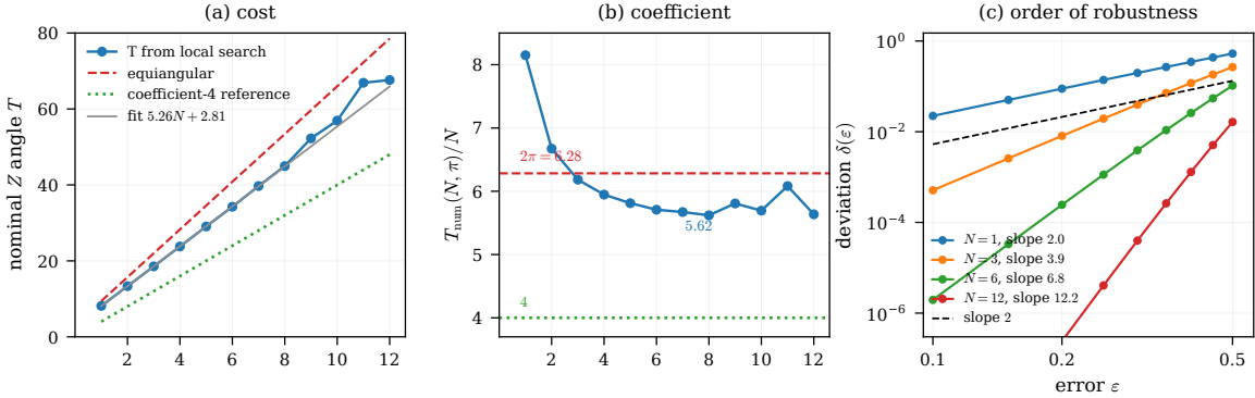
FIG. 1. The same data as Table III. (a) Cost found by the local search, against the reference cost (2N + 1)\pi and the coefficient-4 line 4N ; the straight line is the fit T \approx 5.26N + 2.81 to the branch N \leq 8 , whose residuals are below 0.12. (b) The same cost divided by N ; the horizontal references are the proved lower bound 4 and 2\pi \approx 6.28 , which the values at N = 1, 2 exceed. (c) The deviation \delta(\varepsilon) on a log-log grid for N = 1, 3, 6, 12 , with its local slope; the dashed line has slope 2, the smallest order appearing in the figure, and each curve is drawn only while \delta stays above the round-off floor.
