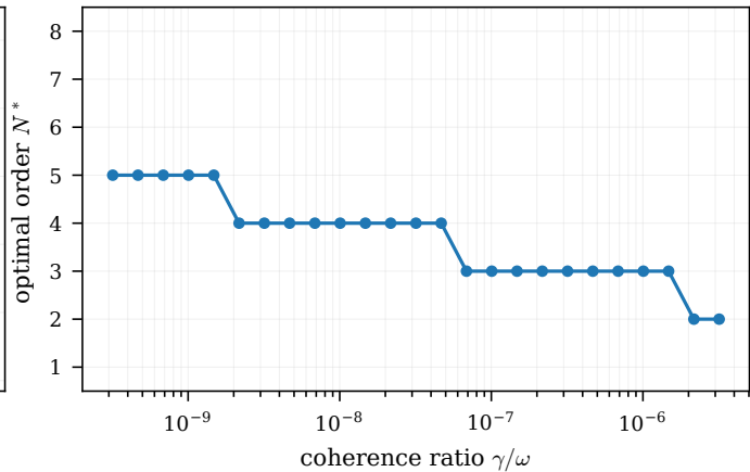
(b) \varepsilon = 0.12 : N^* grows logarithmically
