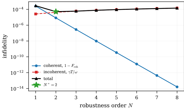
(a) balance at \gamma/\omega = 3 \times 10^{-6} , \varepsilon = 0.12
