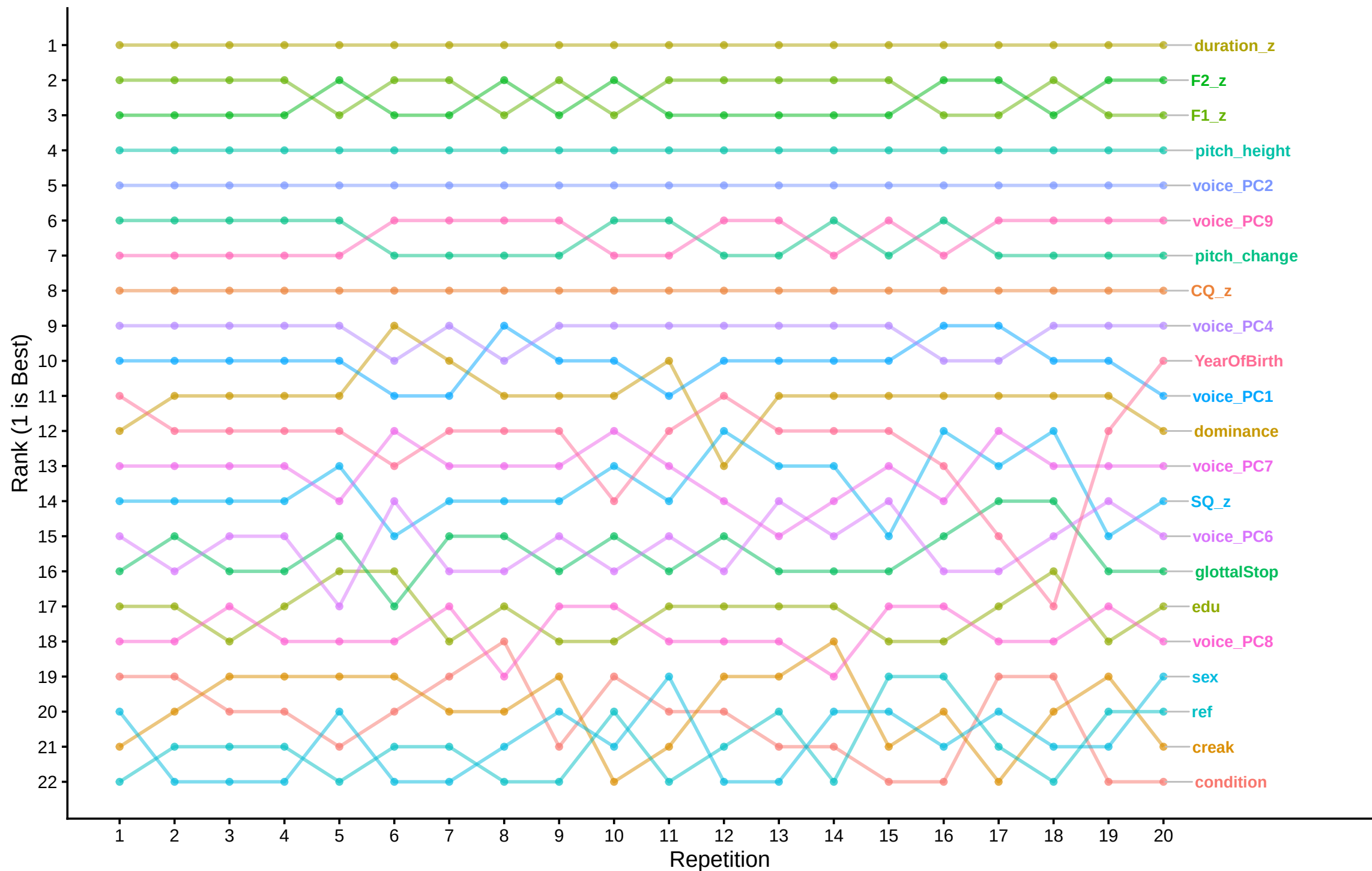
SHAP Feature Ranking Stability
