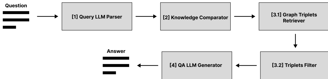
FIGURE 2. High level architecture of proposed QA pipeline for generating answers to the questions based on constructed knowledge graph
