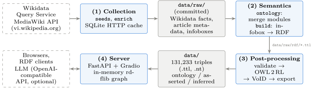
Figure 1: Architecture. Blue boxes are the four layers of the vidbmedia package, gray boxes are files on disk, dashed boxes are external systems. Only layer (1) calls the network.
