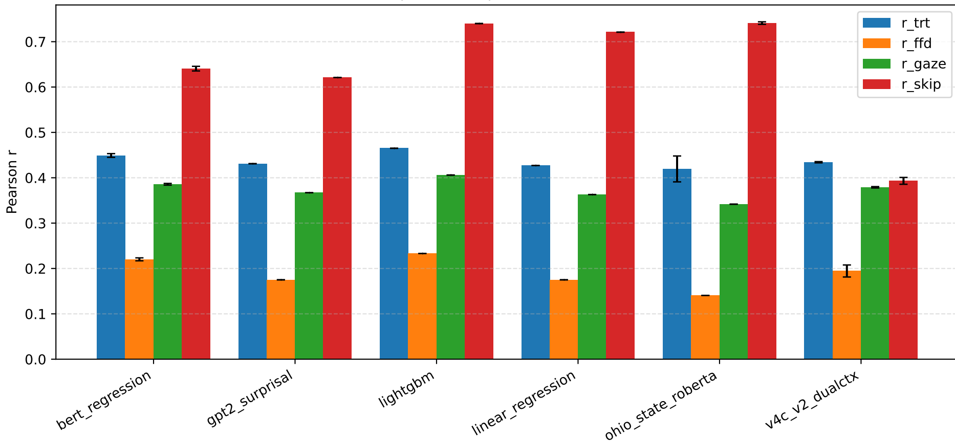
Word-level prediction performance on GECO test
