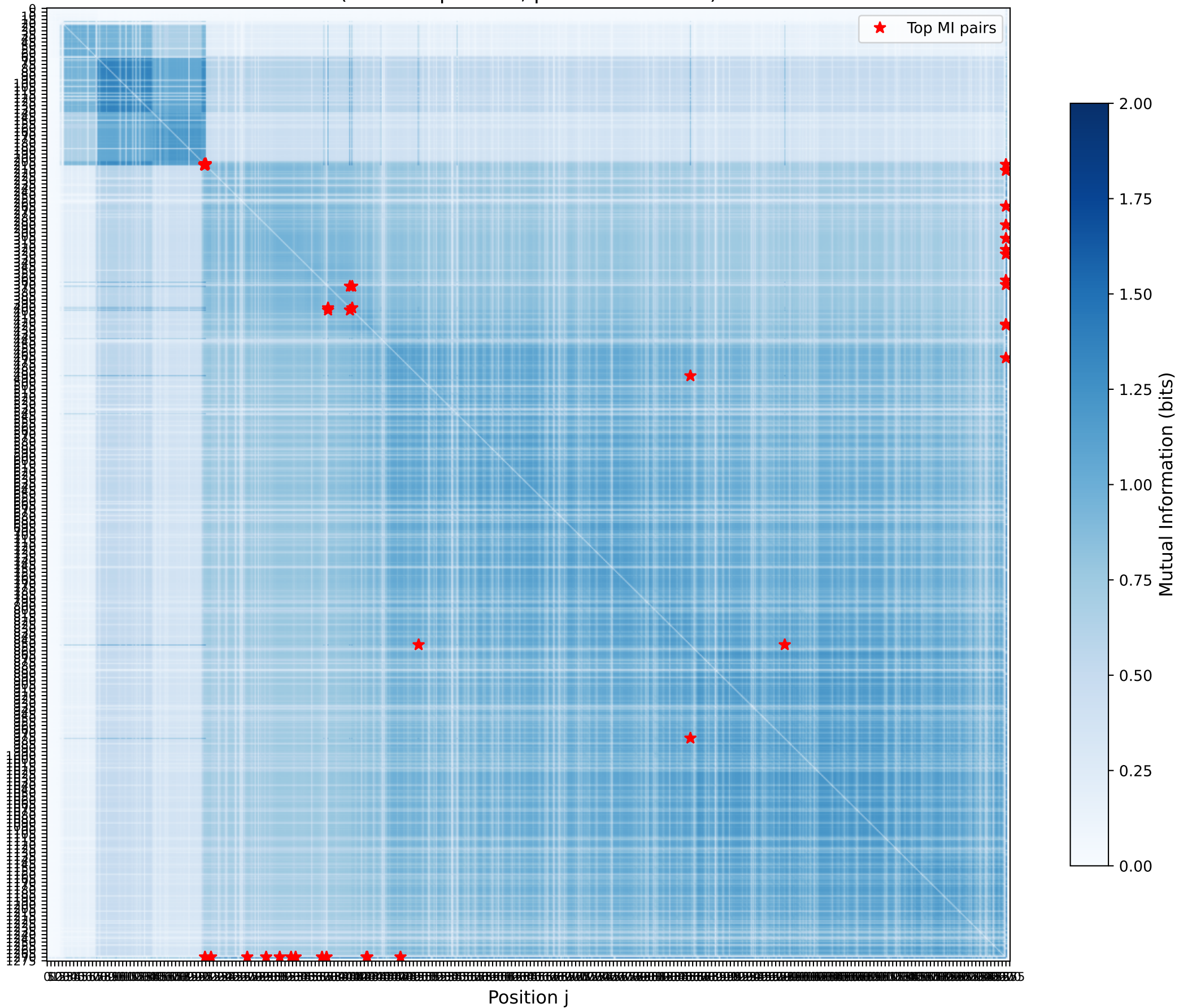
Mutual Information Heatmap - SARS-CoV-2 Spike Protein (1299 sequences, positions 0-1275)
