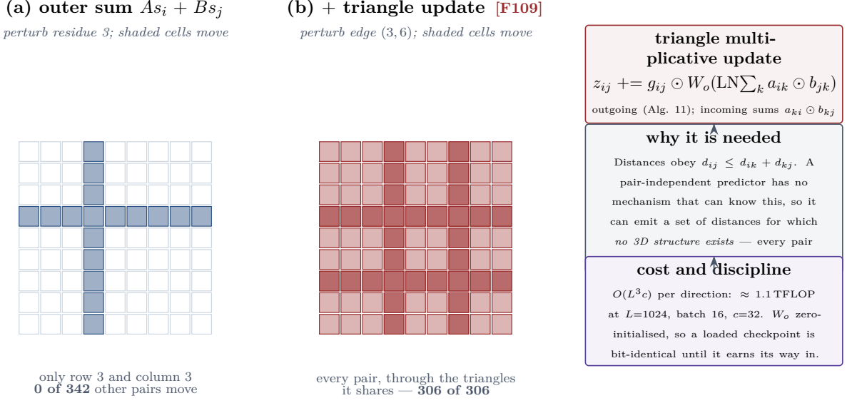
Figure 5: Finding 109. DiffusionPairFeatures is an outer sum, so z_{ij} is a function of its two endpoints and of nothing else. Measured, not inferred: perturb one residue’s hidden state and 0 of 342 pairs that exclude it move. With the triangle update, 306 of 306 do.
