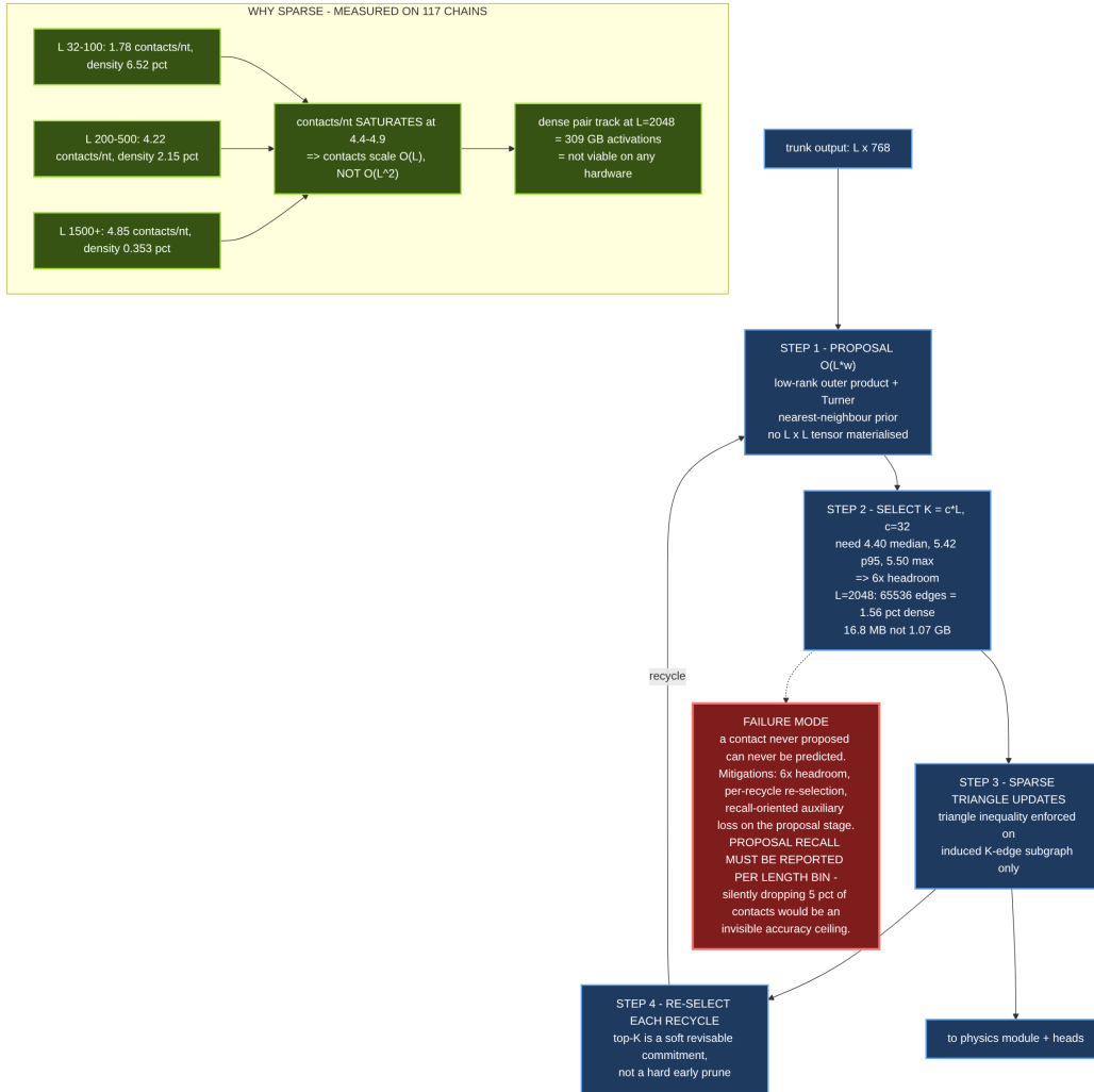
Figure 4: The sparse pair track and its measured justification.
