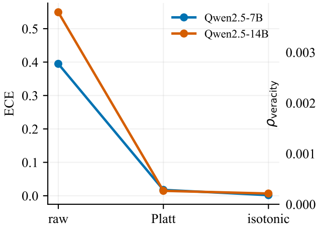
Calibration error drops
