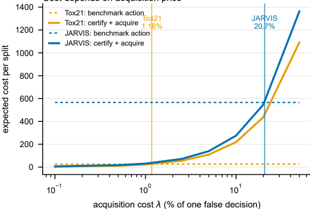
Cost depends on acquisition price
