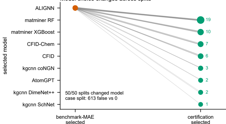
Model choice changes across splits
