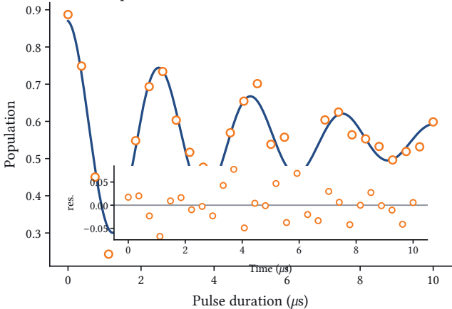
5. Residual plot
