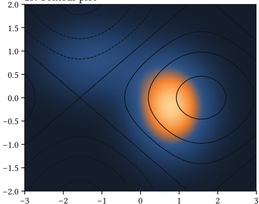
23. Contour plot
