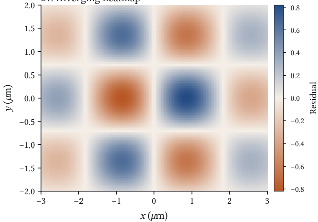
21. Diverging heatmap
