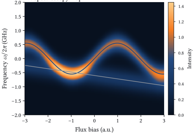
19. Spectroscopy map
