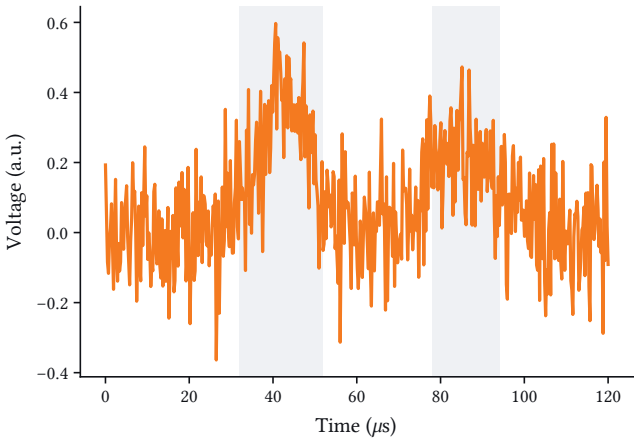
15. Time trace
