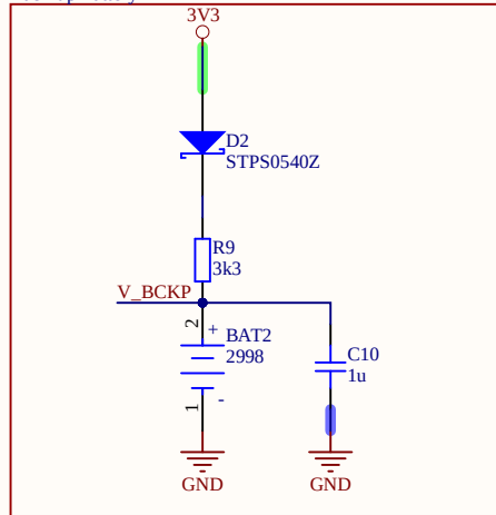
Back-up Battery
