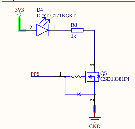
Timepulse LED
