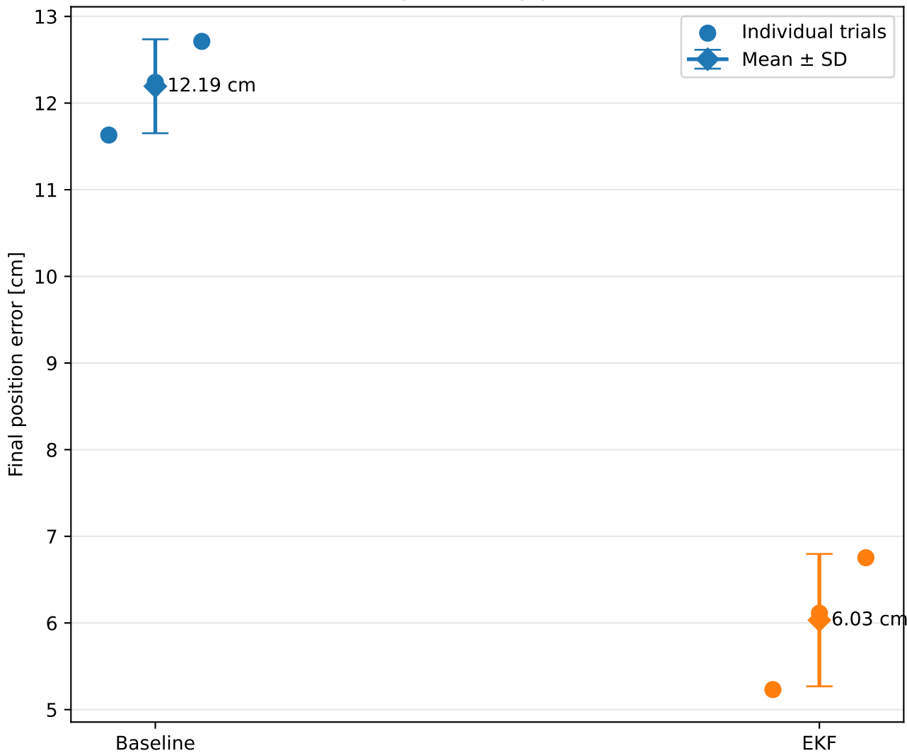
Closed-loop odometry position error
