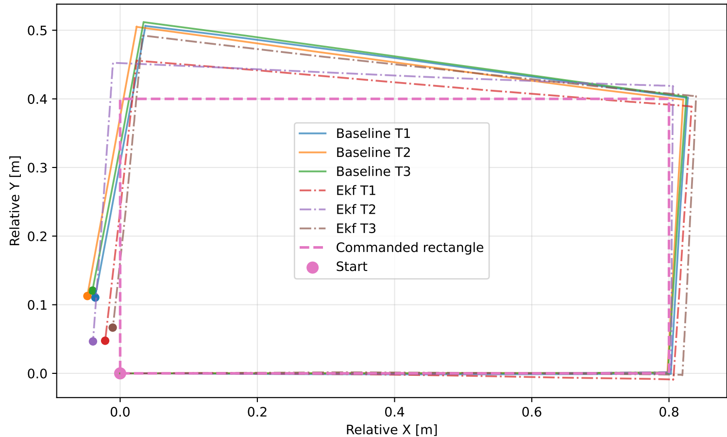
Odometry trajectory: Baseline vs EKF
