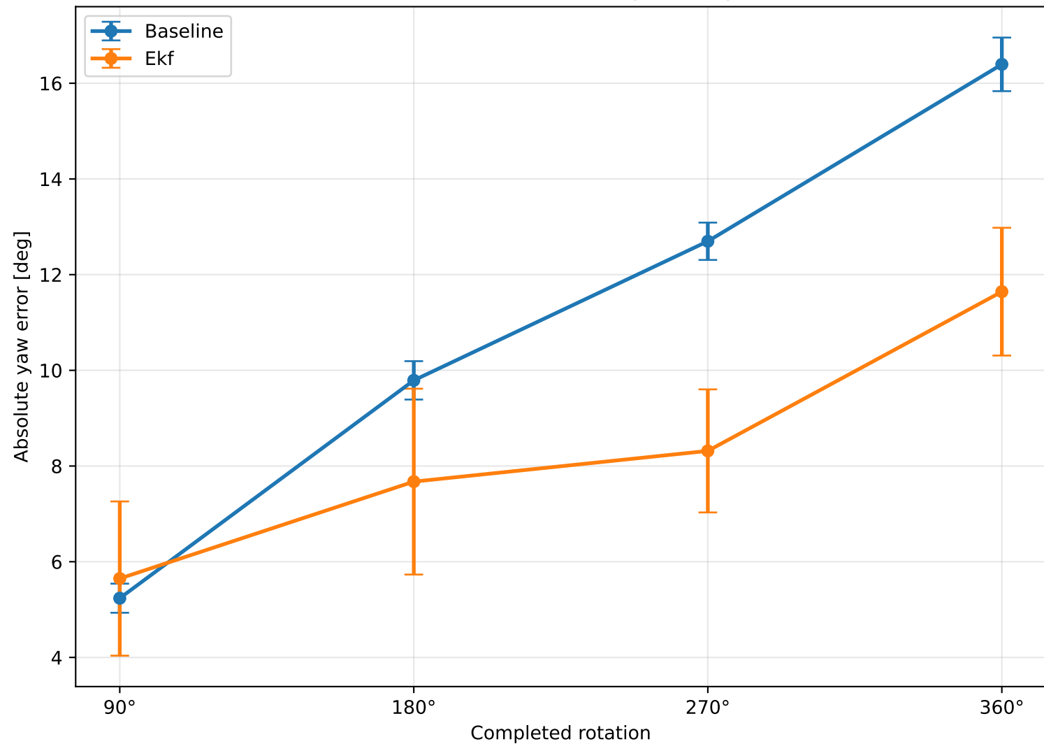
Yaw error accumulation during rectangle turns
