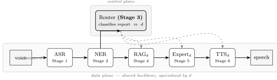
Fig. 1. The specialist-routing cascade. The data plane (bottom) carries the signal \text{voice} \rightarrow \text{ASR} \rightarrow \text{NER} \rightarrow \text{RAG} \rightarrow \text{Expert} \rightarrow \text{TTS} \rightarrow \text{speech} . The control plane (Stage 3) classifies each report into a domain d from the transcript and extracted fields; this single decision conditions (dashed) the evidence partition (Stage 4), the expert persona (Stage 5), and the synthesis voice (Stage 6). The data plane is a shared backbone specialised by d rather than |\mathcal{D}| separate models. All stages run on-device.
