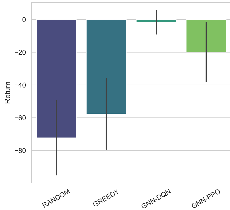
Final Episode Return
