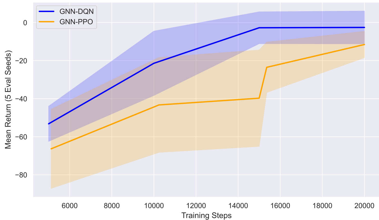
Learning Curve: Episode Return
