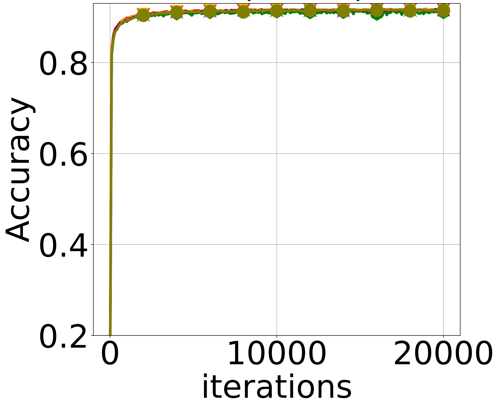
IID (MNIST)
