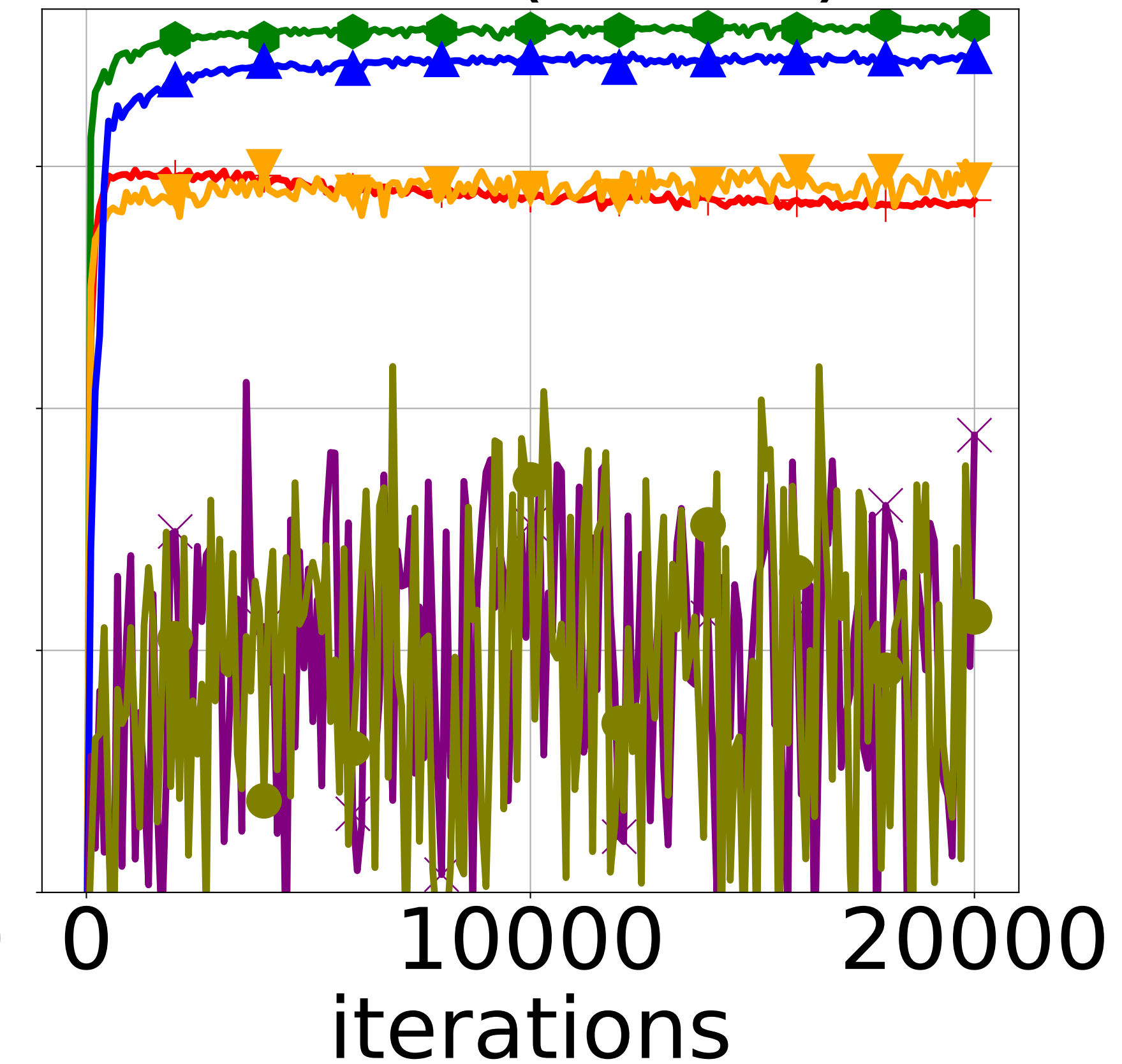
Noniid (MNIST)
