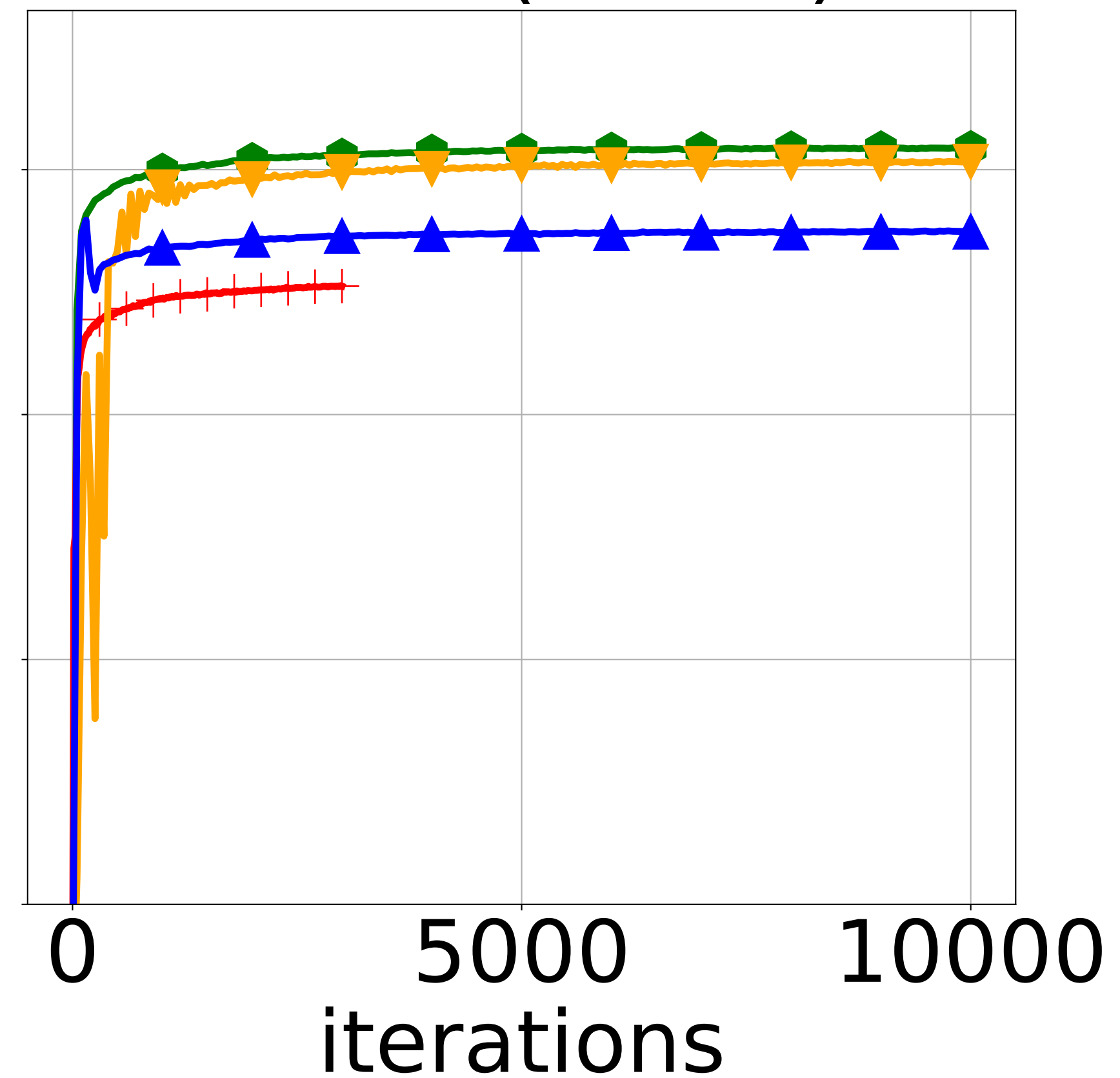
Noniid (MNIST)
