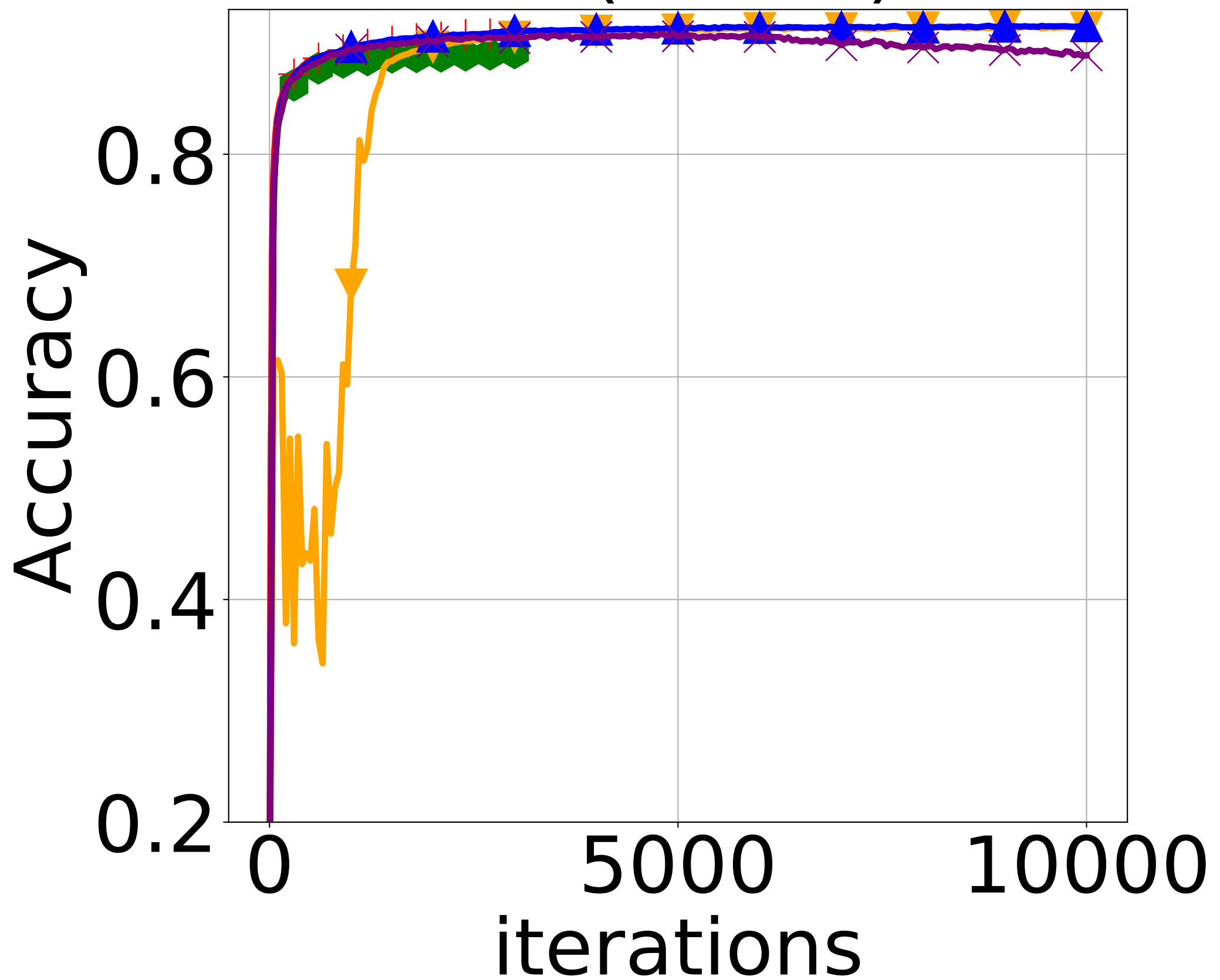
IID (MNIST)
