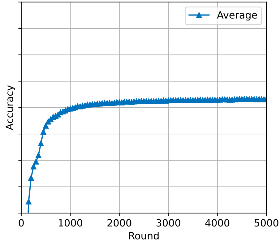
NoAttack attack
