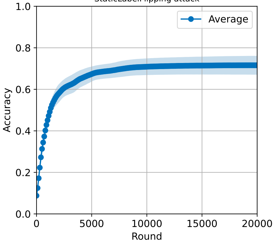
StaticLabelFlipping attack
