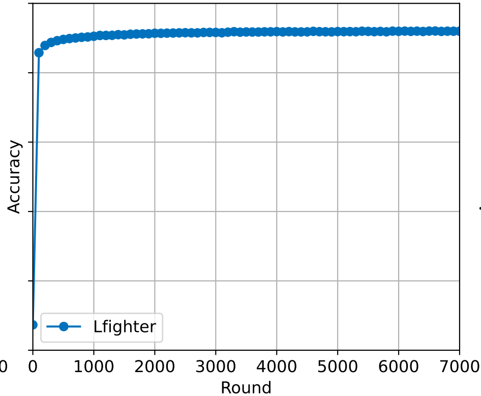
DynamicLabelFlipping attack
