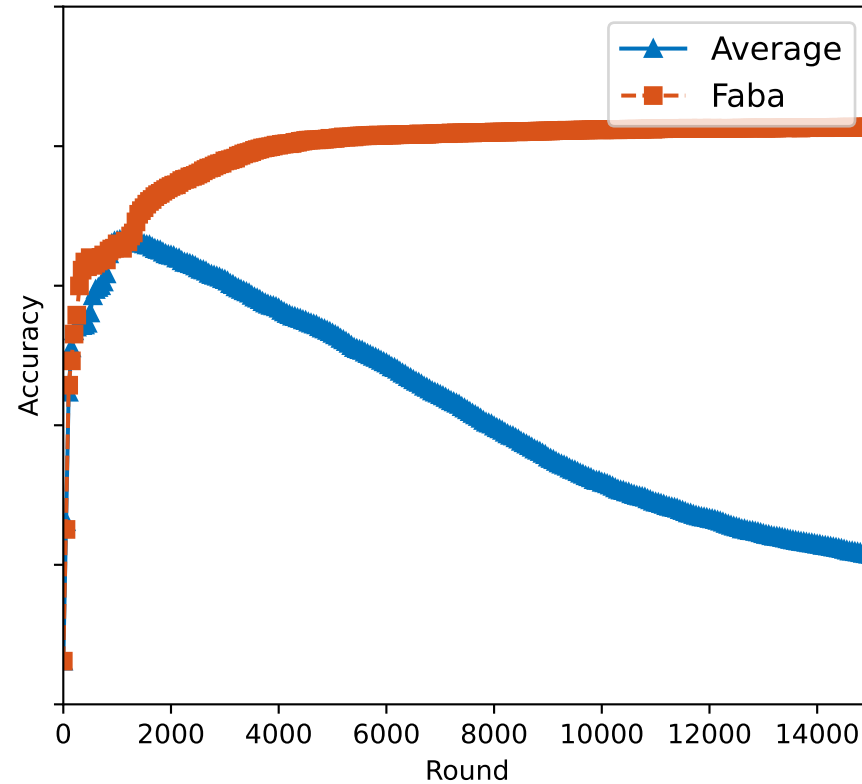
StaticLabelFlipping attack
