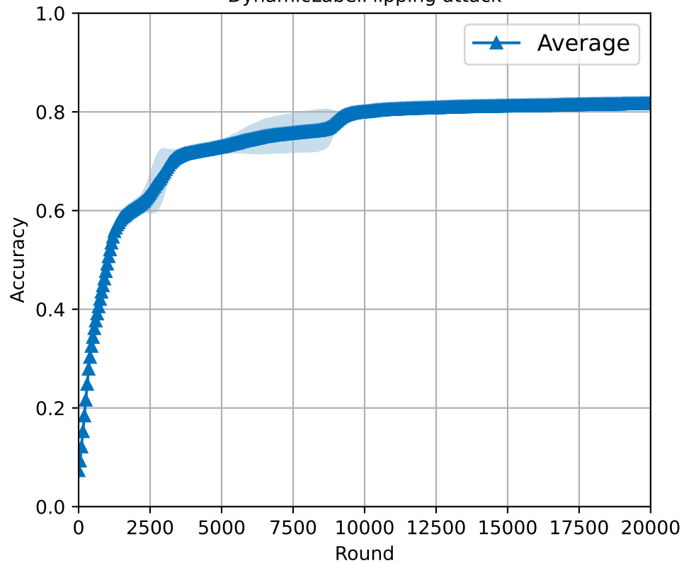
DynamicLabelFlipping attack
