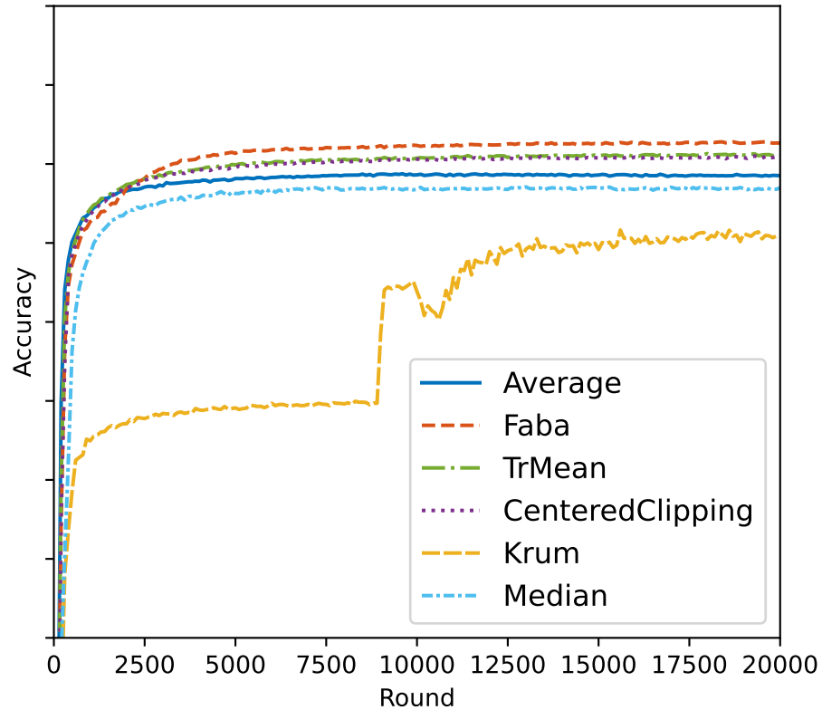
StaticLabelFlipping attack
