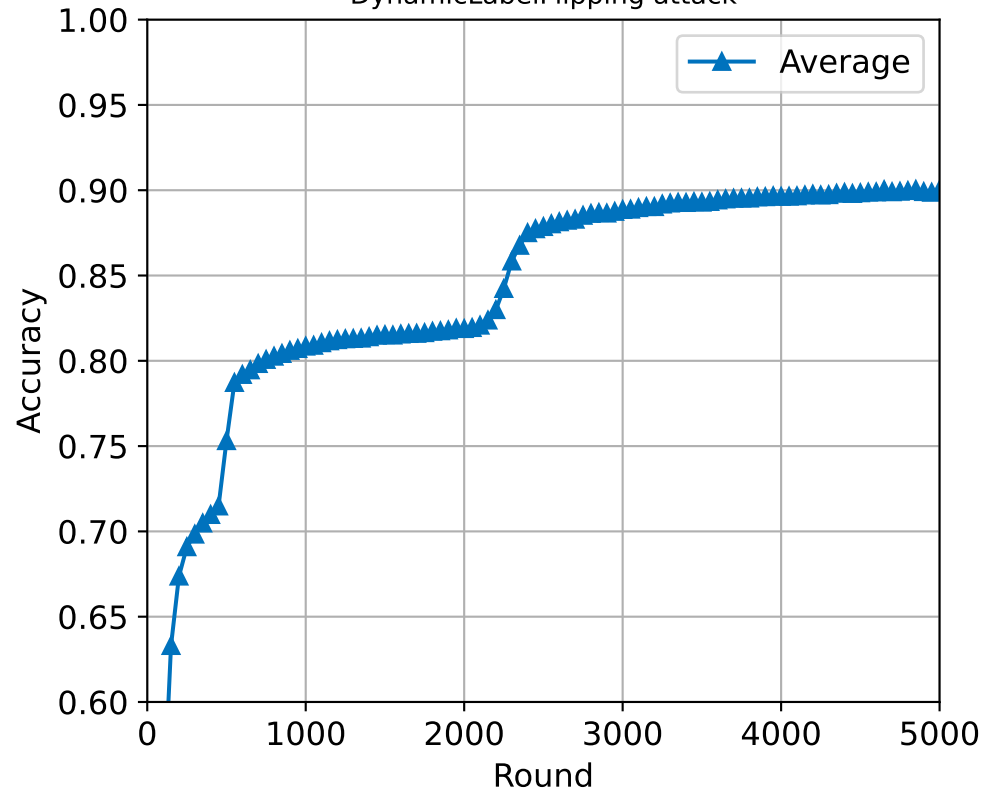
DynamicLabelFlipping attack
