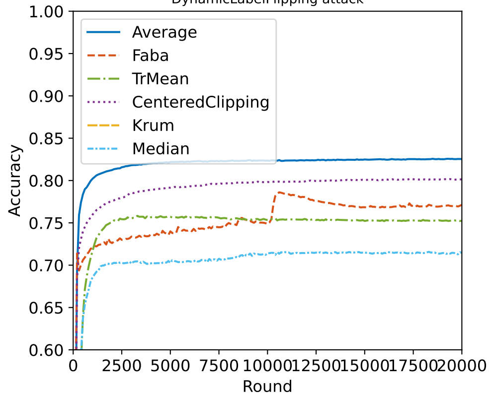
DynamicLabelFlipping attack
