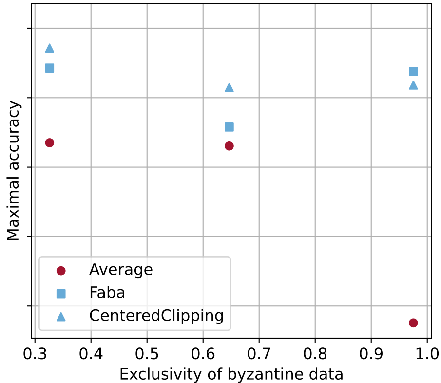
StaticLabelFlipping attack
