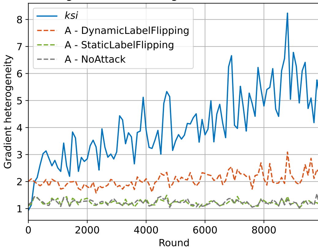
Raw gradient scatterings, iid-None distribution
