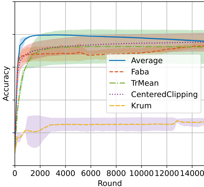
StaticLabelFlipping attack
