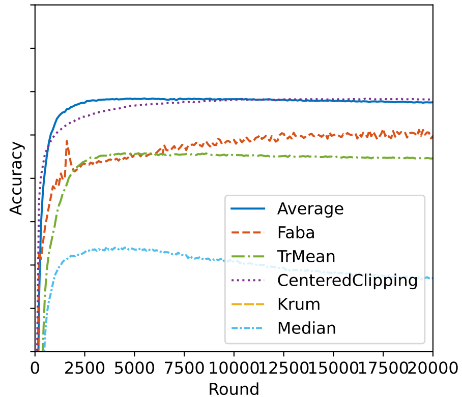
NoAttack attack
