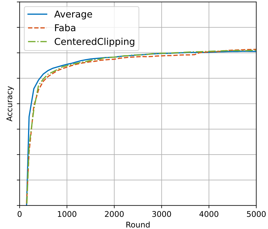
NoAttack attack
