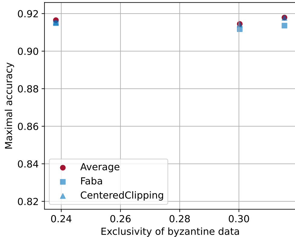
DynamicLabelFlipping attack
