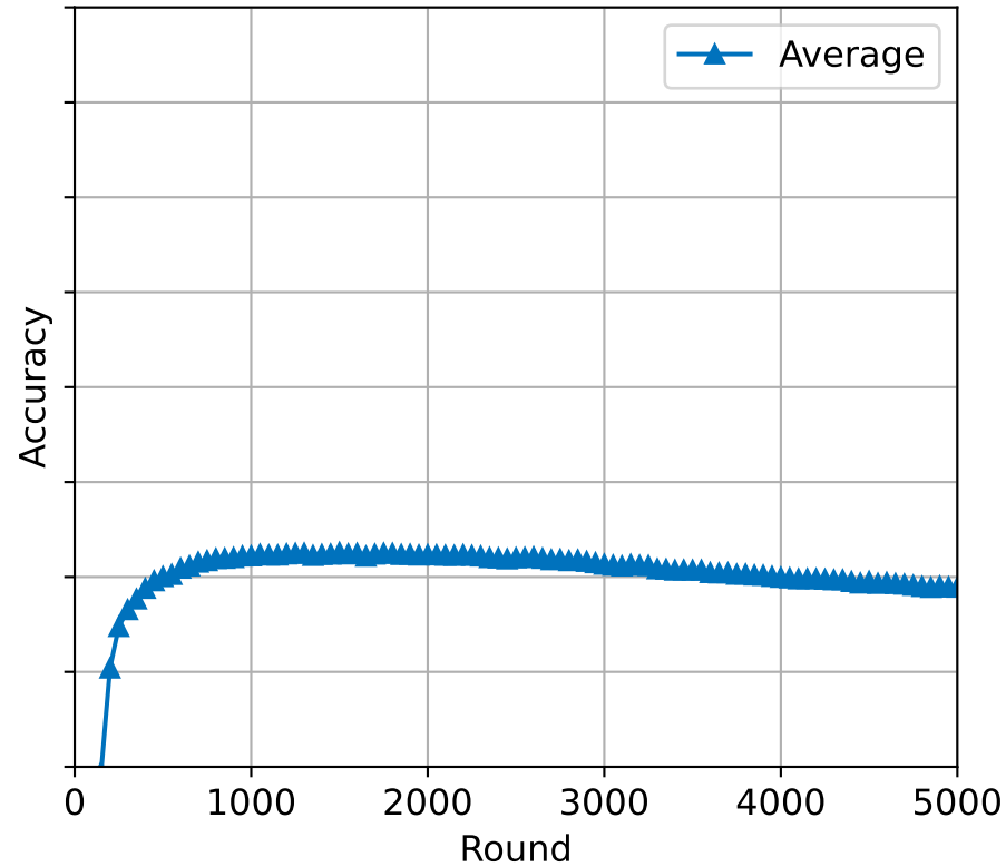
StaticLabelFlipping attack
