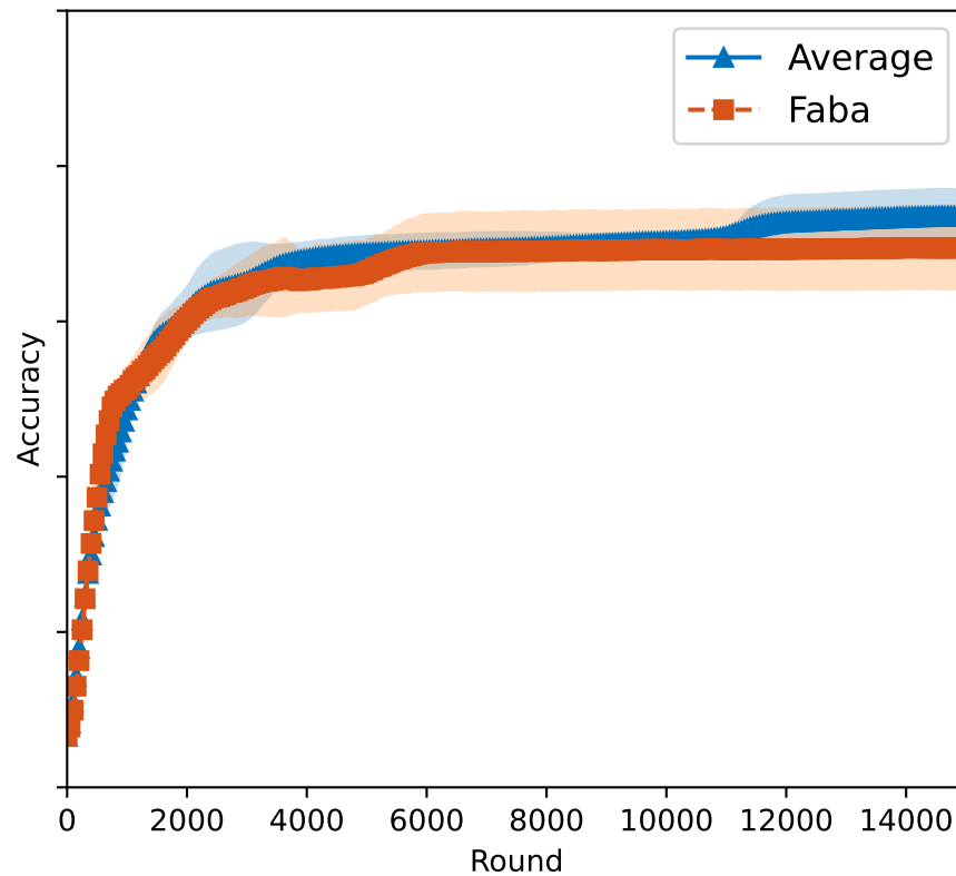
StaticLabelFlipping attack
