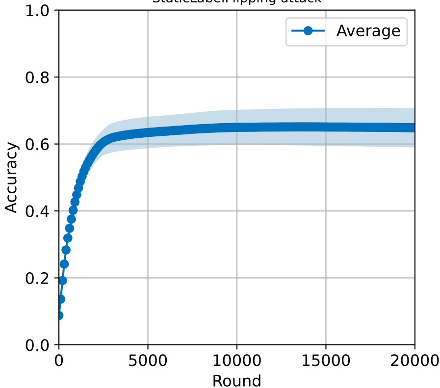
StaticLabelFlipping attack
