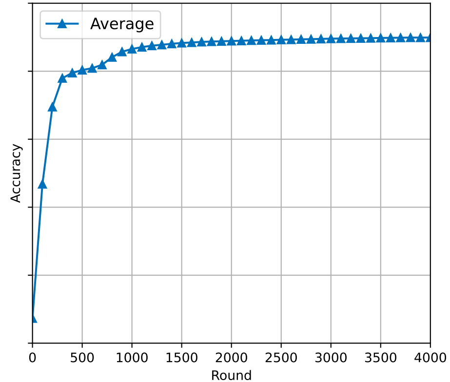
NoAttack attack
