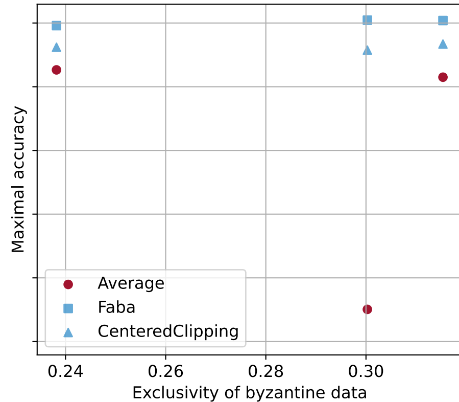
NoAttack attack
