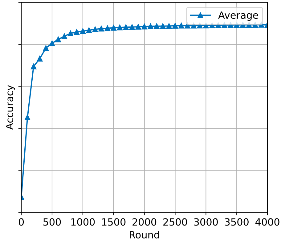
NoAttack attack
