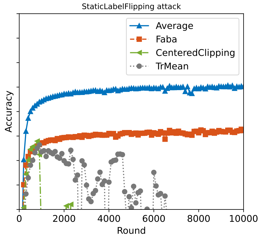
Accuracy paths, distribution: extreme_niid_modified_None
