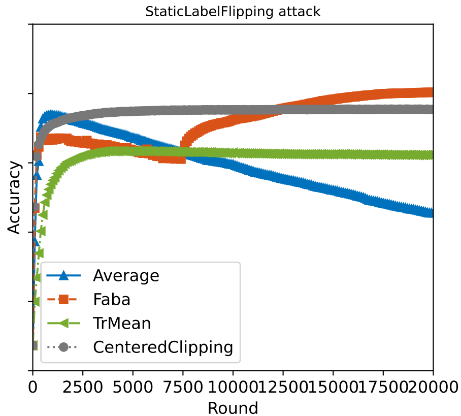
Accuracy paths, distribution: dirichlet_niid_modified_0.03
