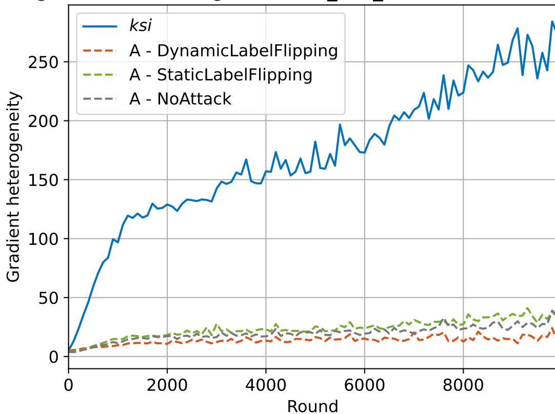
Raw gradient scatterings, dirichlet_niid_modified-0.03 distribution
