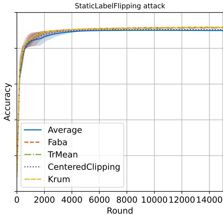
Accuracy paths, distribution: iid_None
