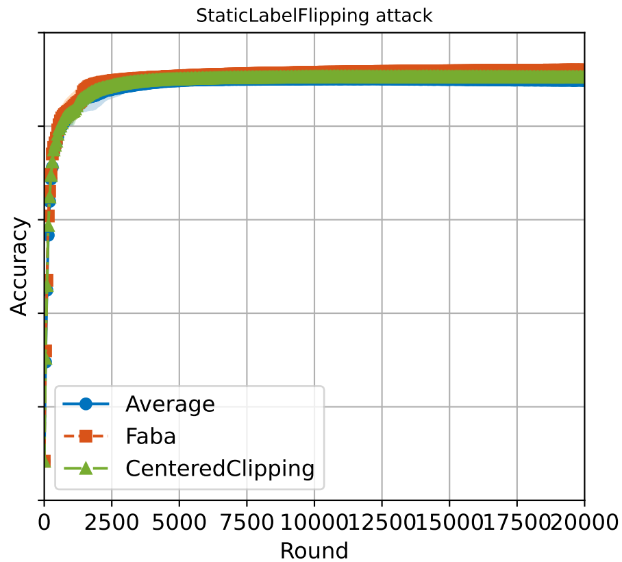
Accuracy paths, distribution: iid_None
