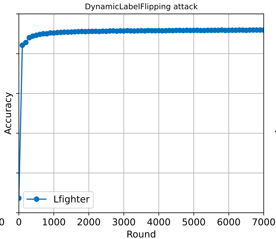
Accuracy paths, distribution: dirichlet_niid_modified_1.0
