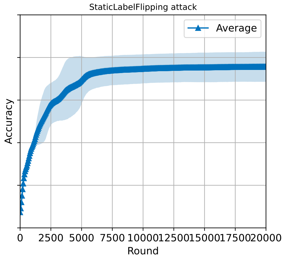
Accuracy paths, distribution: dirichlet_niid_modified_0.05
