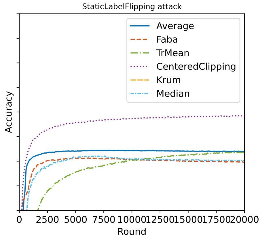
Accuracy paths, distribution: dirichlet_niid_modified_0.1
