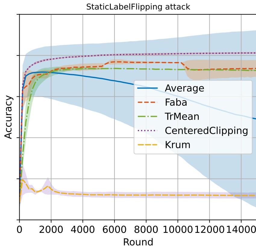
Accuracy paths, distribution: dirichlet_niid_modified_0.01
