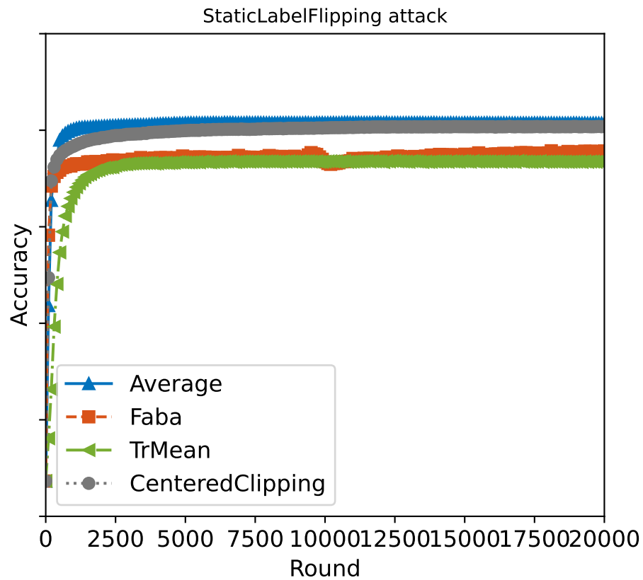
Accuracy paths, distribution: extreme_niid_modified_None
