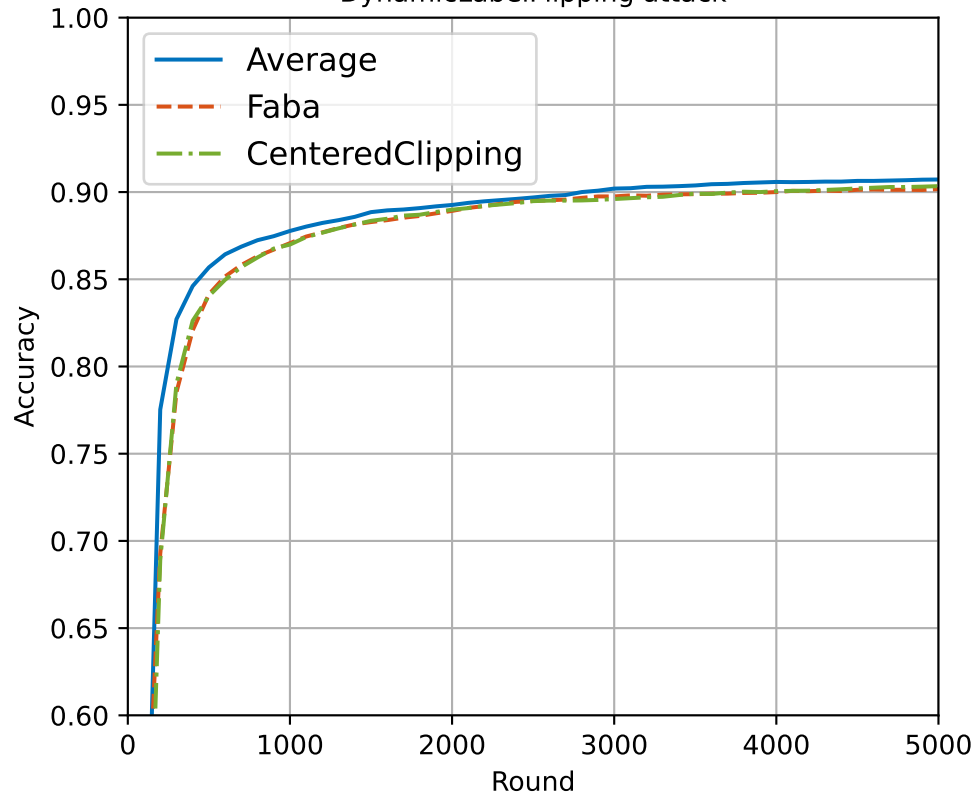
DynamicLabelFlipping attack
