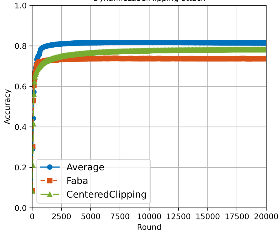
DynamicLabelFlipping attack
