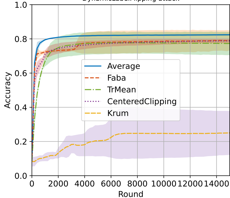
DynamicLabelFlipping attack
