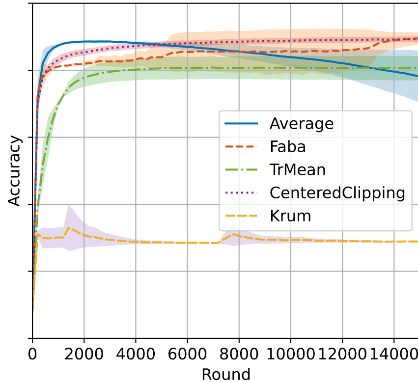
NoAttack attack
