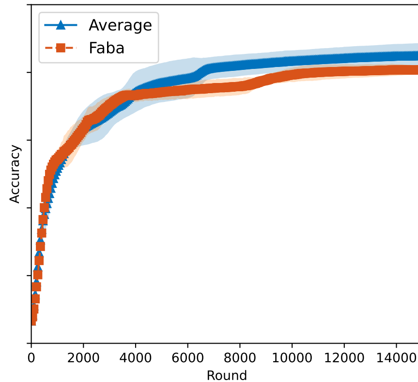
NoAttack attack
