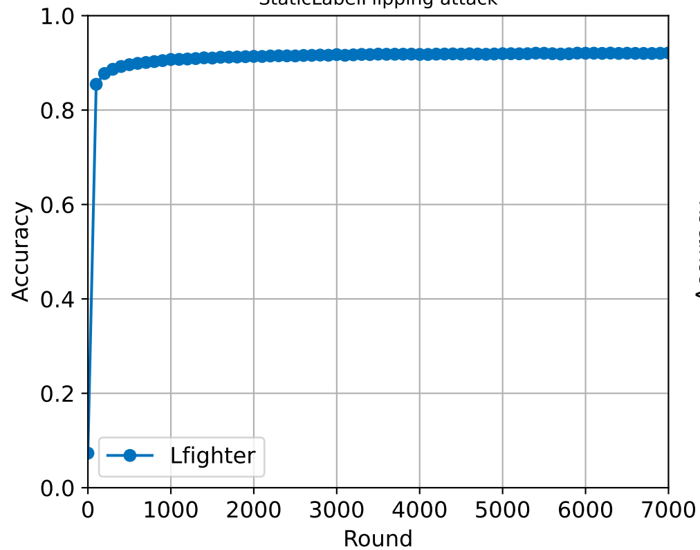
StaticLabelFlipping attack
