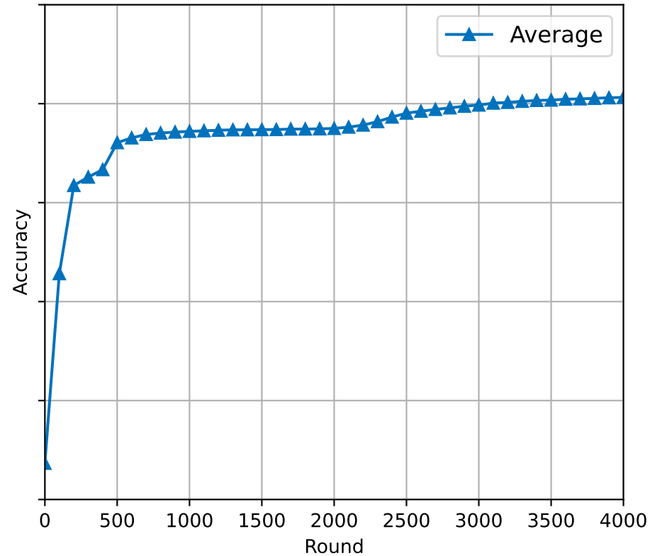
StaticLabelFlipping attack
