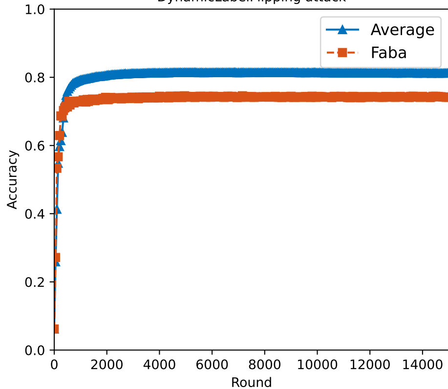
DynamicLabelFlipping attack
