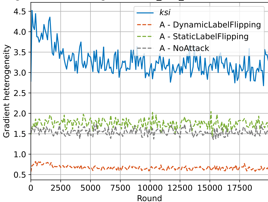
Raw gradient scatterings, dirichlet_niid_modified-0.05 distribution
