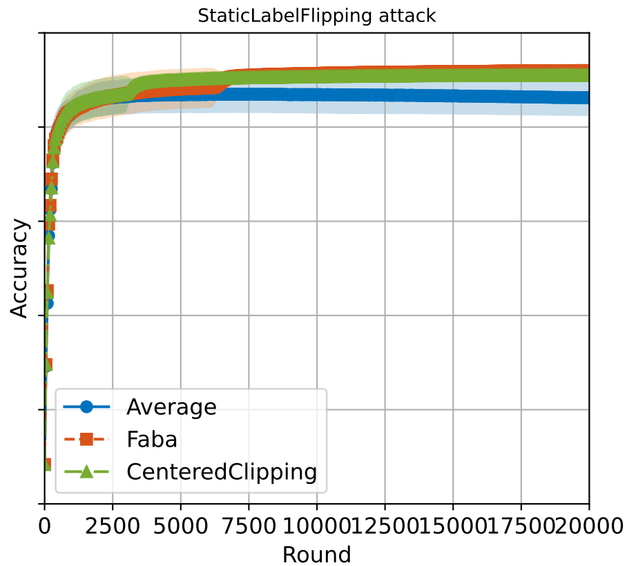
Accuracy paths, distribution: dirichlet_niid_modified_1.0
