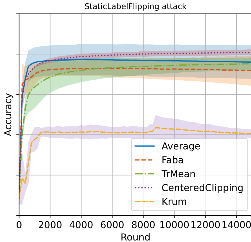
Accuracy paths, distribution: dirichlet_niid_modified_0.1
