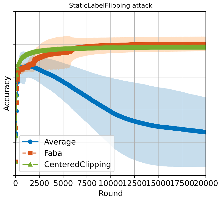
Accuracy paths, distribution: dirichlet_niid_modified_0.01
