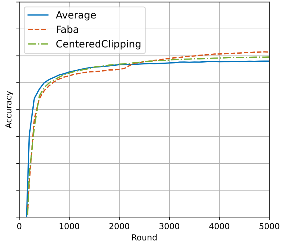
StaticLabelFlipping attack
