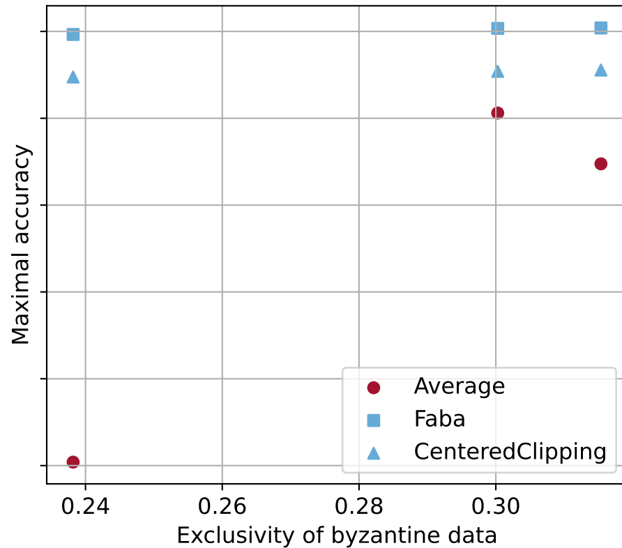
StaticLabelFlipping attack
