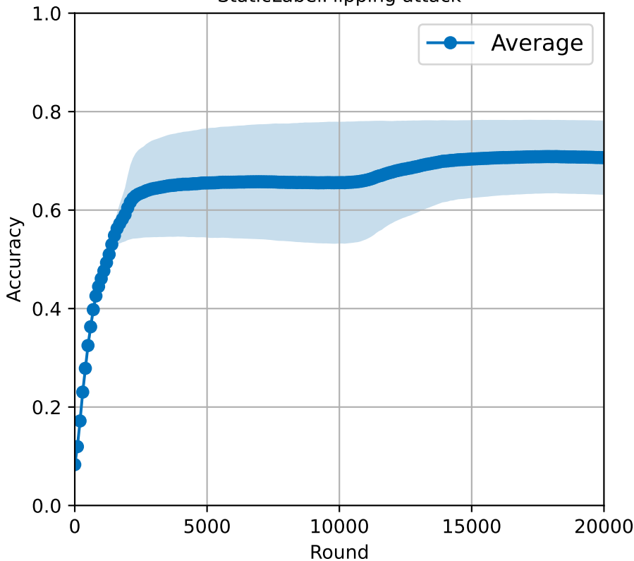
StaticLabelFlipping attack
