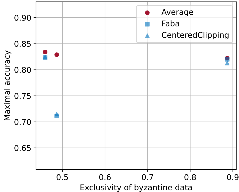
DynamicLabelFlipping attack
