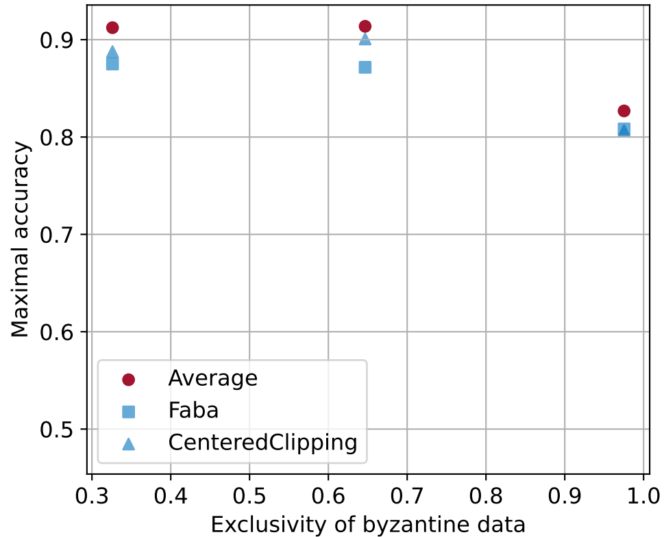
DynamicLabelFlipping attack
