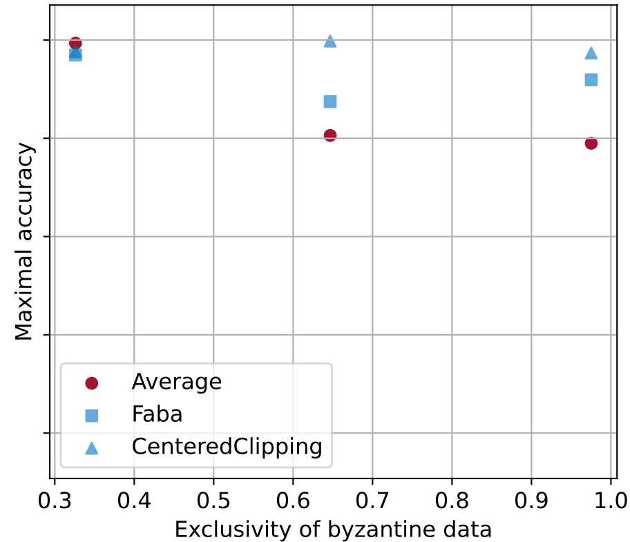
NoAttack attack
