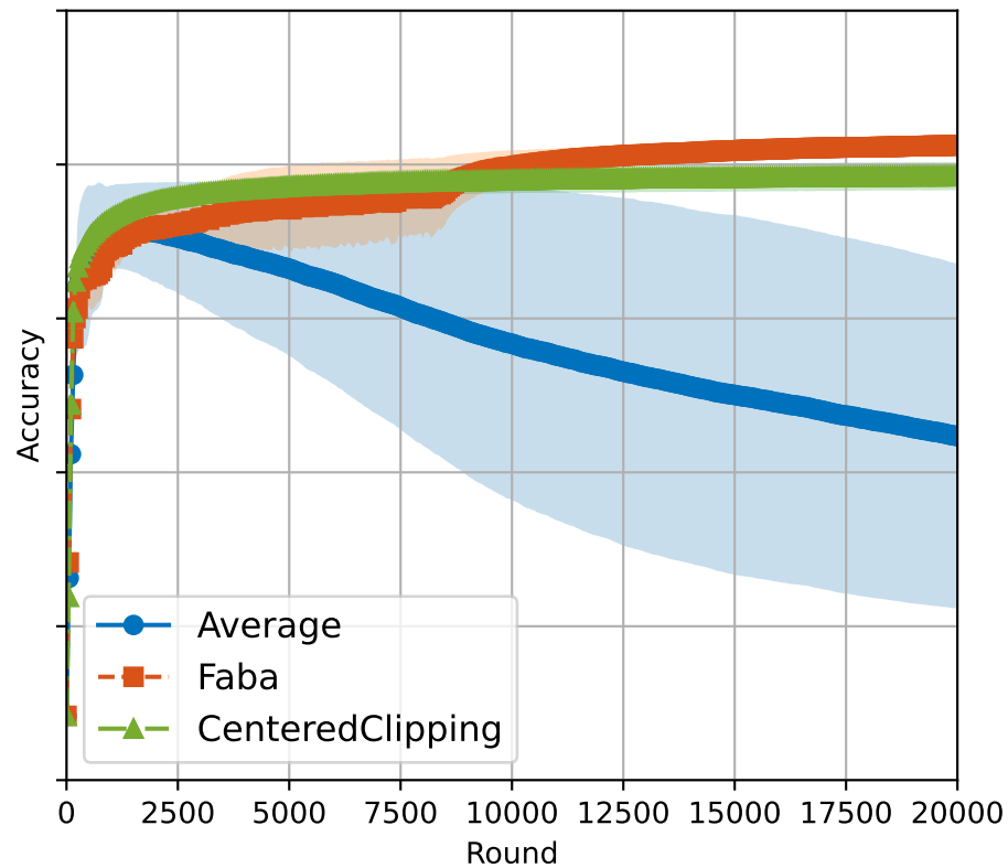
StaticLabelFlipping attack
