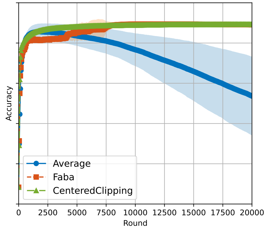
NoAttack attack
