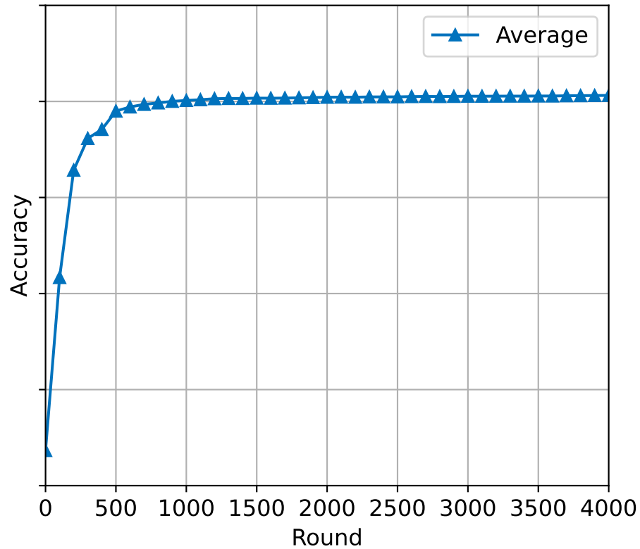
StaticLabelFlipping attack
