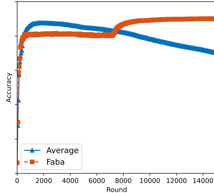
NoAttack attack
