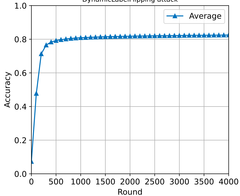
DynamicLabelFlipping attack
