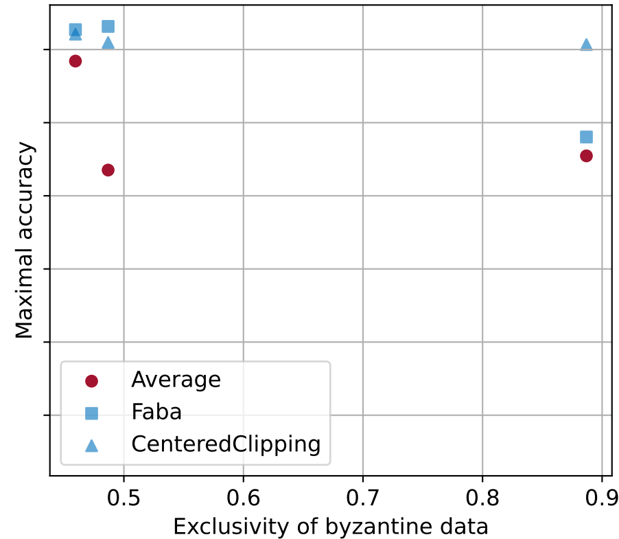
NoAttack attack
