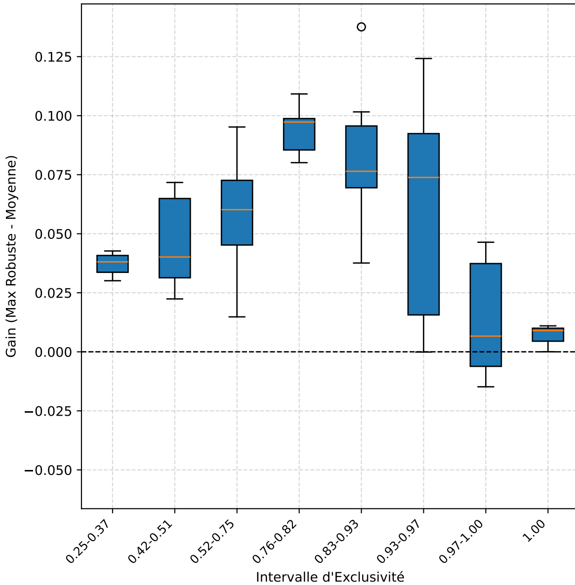
StaticLabelFlipping
