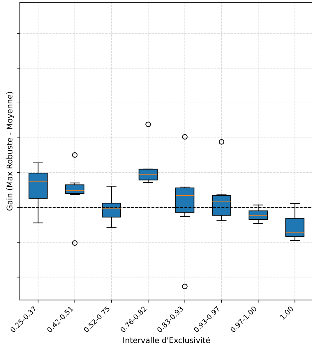
DynamicLabelFlipping
