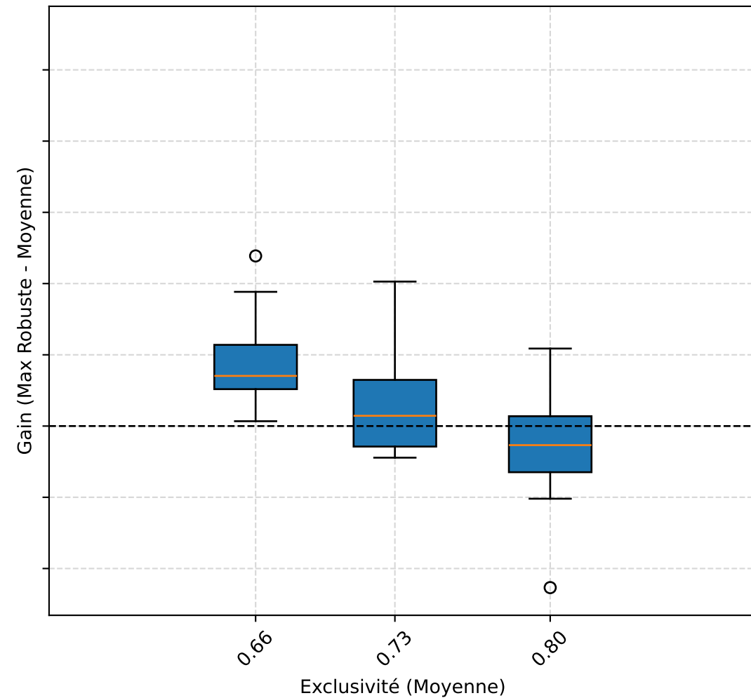
DynamicLabelFlipping
