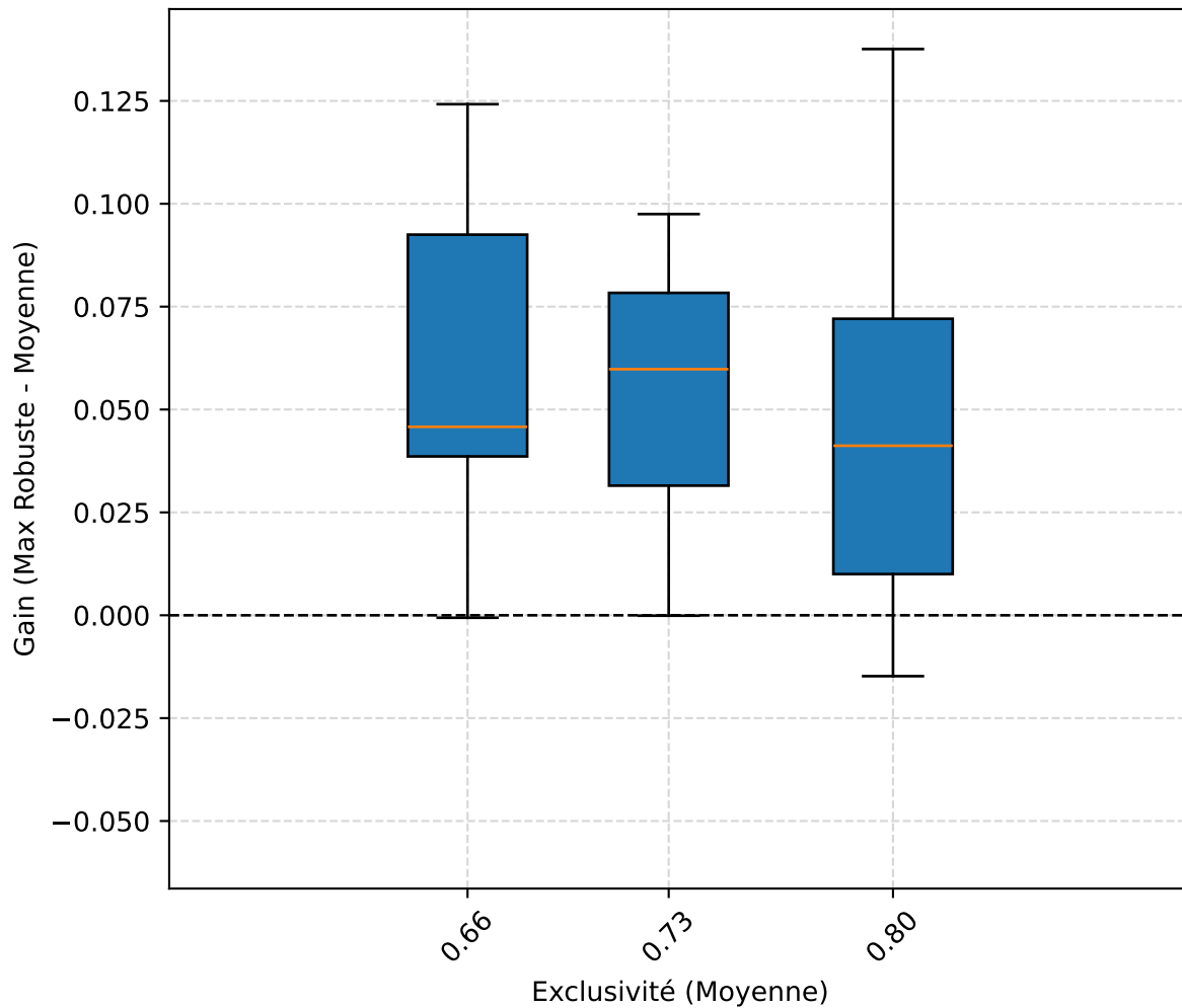
StaticLabelFlipping
