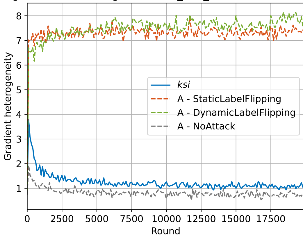
Raw gradient scatterings, dirichlet_niid_modified-1.0 distributio
