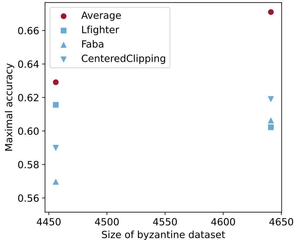
DynamicLabelFlipping attack
