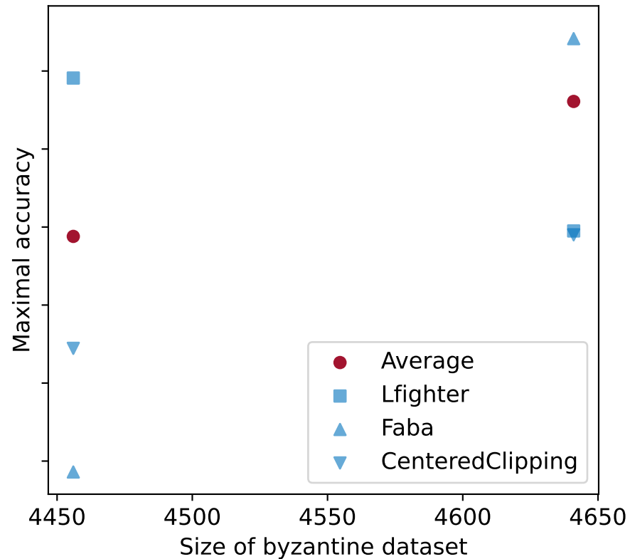
StaticLabelFlipping attack
